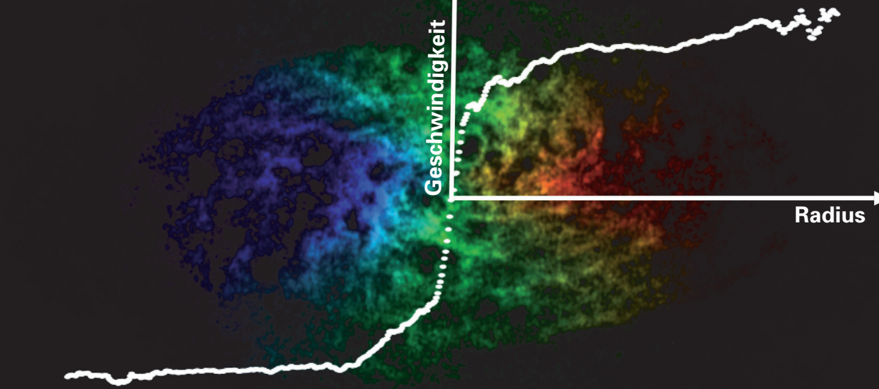
NGC 2403 – Rotation
