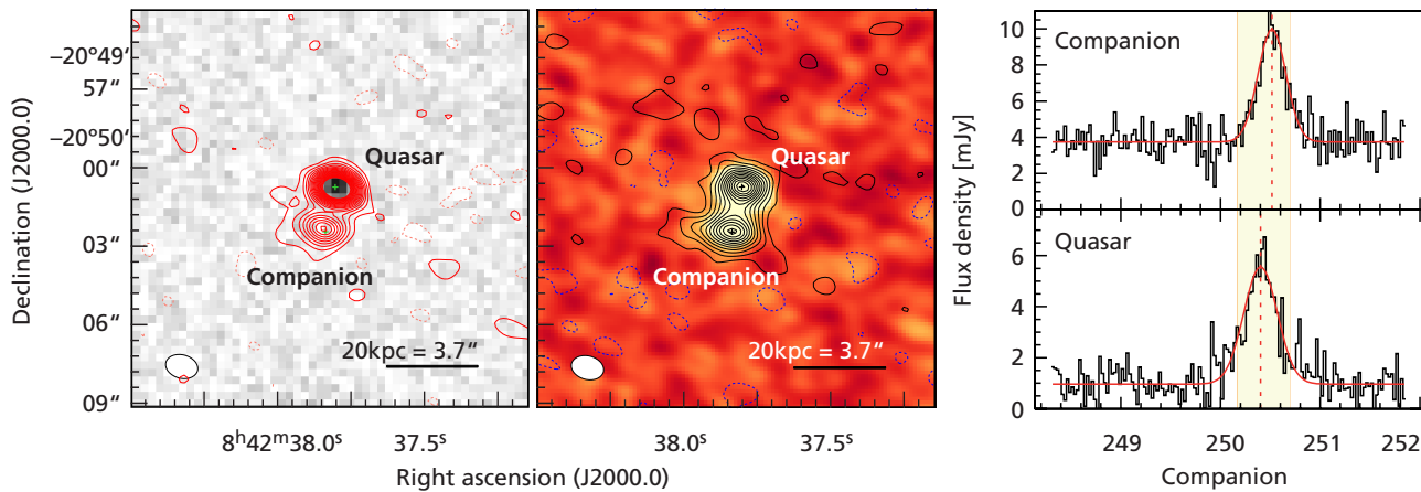
PJ308-21, z = 6.2342 , \Delta v = 590 \text{ km s}^{-1}
