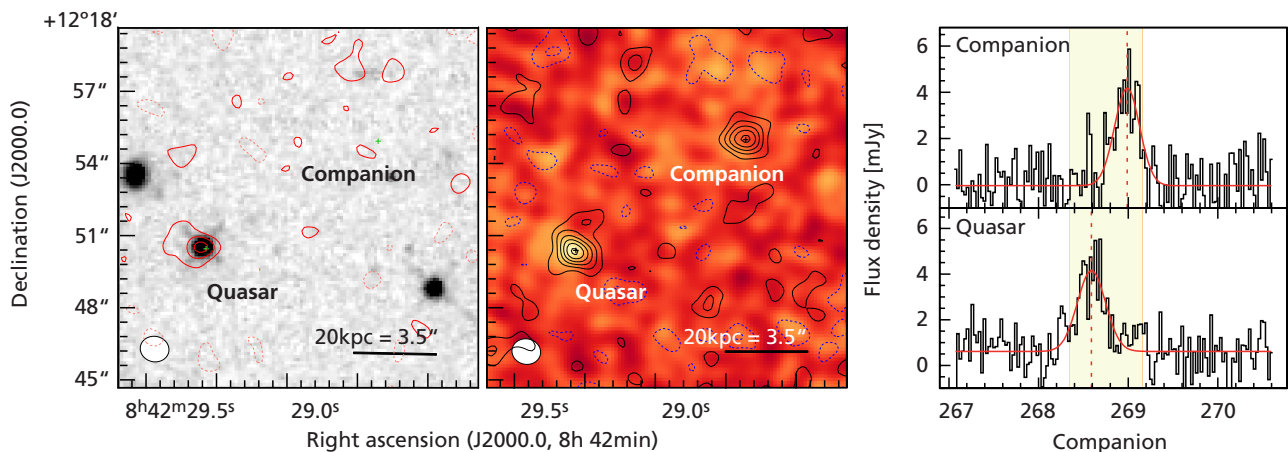
J2100-1715, z = 6.0806 , \Delta v = -40 \text{ km s}^{-1}
