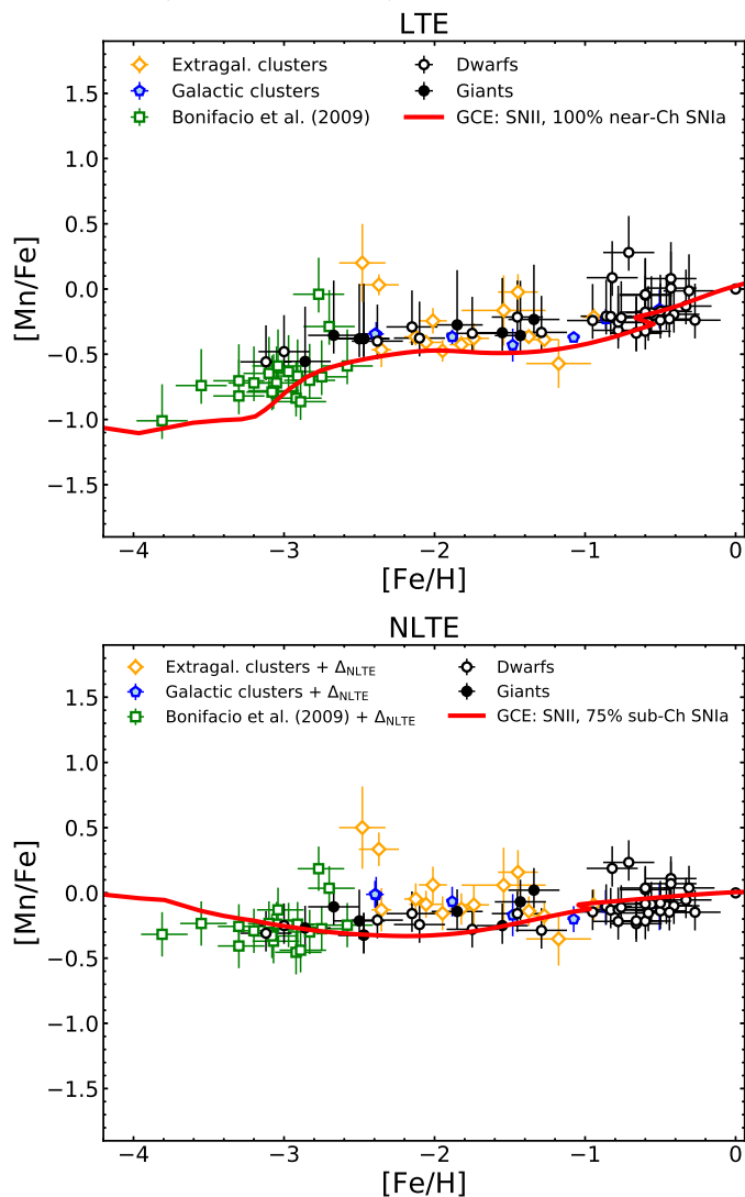
Fig. 2. Manganese abundance ratios as a function of metallicity. Top panel: LTE data are presented with different symbols; the line shows the results of the GCE model with yield for SNe II taken from Woosley & Weaver (1995), including only near- M_{\text{ch}} SNe Ia with by Iwamoto et al. (1999). Bottom panel: NLTE data. The GCE model presented here adopts the yields by Kobayashi et al. (2011) for SNe II and includes 25% of near- M_{\text{ch}} and 75% of sub- M_{\text{ch}} SNe Ia.
