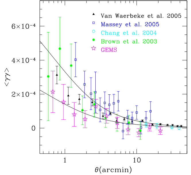
Figure 15. Comparison of the total shear correlation function E[\gamma\gamma]_\theta as measured from GEMS along with the most up-to-date shear correlation measurements from the other groups indicated. Overplotted are theoretical \Lambda CDM models for a z_m = 1 survey with \sigma_8 = 0.7 (lower) and \sigma_8 = 1.0 (upper). Note all data points and errors have been scaled to a z_m = 1 survey using a z_m^2 redshift scaling.
