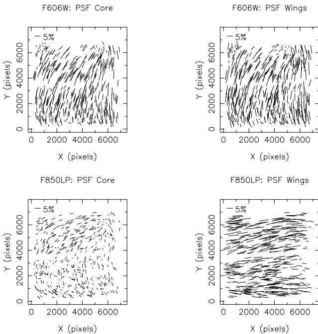
Figure 1. The anisotropic ACS PSF measured from stellar sources in F606W images (upper panels) and F850LP images (lower panels). The stellar ellipticity \varepsilon^* plotted has been measured using two differently scaled weight functions W(r_g) ; left panels r_g = 2.5 pixel (PSF core distortion), right panels r_g = 7 pixel (PSF wing distortion). The 5 per cent bar in the upper left corner of each panel shows the scale, which is the same for each panel.
