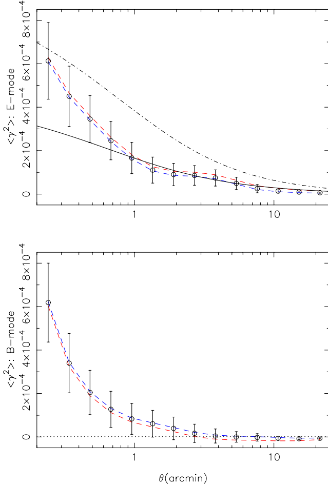
Figure 12. E/B mode decomposition of the shear variance. The upper panel shows \langle \gamma^2 \rangle_\theta^E and the fiducial \Lambda CDM theoretical ( \gamma^2 ) model (solid) where \sigma_8 = 0.7 and the median source redshift z_m = 1.0 . The lower panel shows \langle \gamma^2 \rangle_\theta^B that is consistent with zero on angular scales \theta > 1.5 arcmin. Using a different fiducial \Lambda CDM cosmological model to calculate \langle \gamma^2 \rangle_\theta^{EB} has a small effect (at the level of 3 \times 10^{-5} ) which can be seen from the dotted curves where we have assumed \sigma_8 = 0.6 (lower curve E-mode, upper curve B-mode) and \sigma_8 = 1.0 (upper curve E-mode, lower curve B-mode). The significant non-lensing B-modes at \theta < 1.5 arcmin indicate residual small-scale systematics that, with the shear variance statistic, are included at all angular scales. These non-lensing distortions also contribute to the measured E-mode making the signal appear to favour a high value for \sigma_8 (upper panel: \Lambda CDM \sigma_8 = 1.0 theoretical model overplotted dot-dashed).
