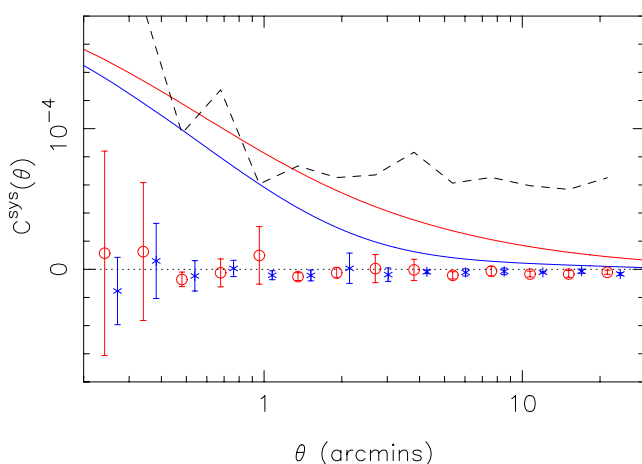
Figure 9. Star–galaxy cross-correlation functions C_{ii}^{\text{sys}} (circles) and C_{rr}^{\text{sys}} (crosses) compared to theoretical galaxy–galaxy shear correlation functions \langle \gamma_r \gamma_r \rangle_\theta (upper curve) and \langle \gamma_t \gamma_t \rangle_\theta (lower curve) with z_m = 1.0 , \Omega_m = 0.3 , and \sigma_8 = 0.7 . For comparison we also measure the star–galaxy cross-correlation in the absence of PSF corrections, shown dashed, where for clarity we plot \frac{1}{2}(C_{ii}^{\text{sys}} + C_{rr}^{\text{sys}}) .
