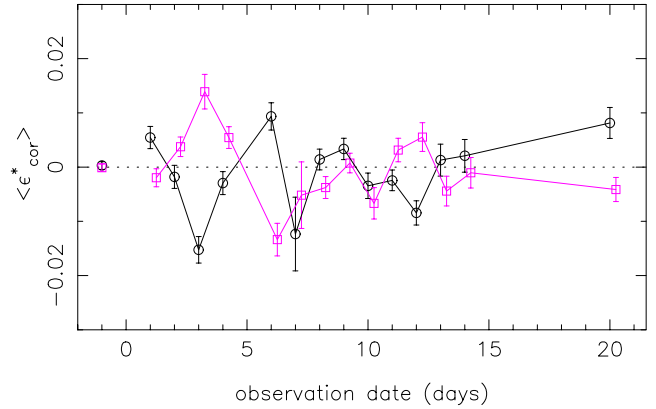
Figure 5. The F606W corrected stellar ellipticity parameters \epsilon_1^{\text{cor}*} (circles) and \epsilon_2^{\text{cor}*} (squares) averaged across the full ACS field of view as a function of observation date. The corrected stellar ellipticity averages to zero over the whole data set as shown by the isolated points on the far left of the plot. In general the PSF correction works well reducing the corrected ellipticity as a function of observation date close to zero, and significantly reducing the scatter (i.e removing the anisotropy) seen in Fig. 4 (plotted on a different scale). There is, however, the occasional case where the stellar ellipticity is significantly different from zero showing that the semi-time-dependent modelling is only a partial solution for time-varying PSF modelling. The errors plotted are the errors on the mean corrected stellar ellipticity.
