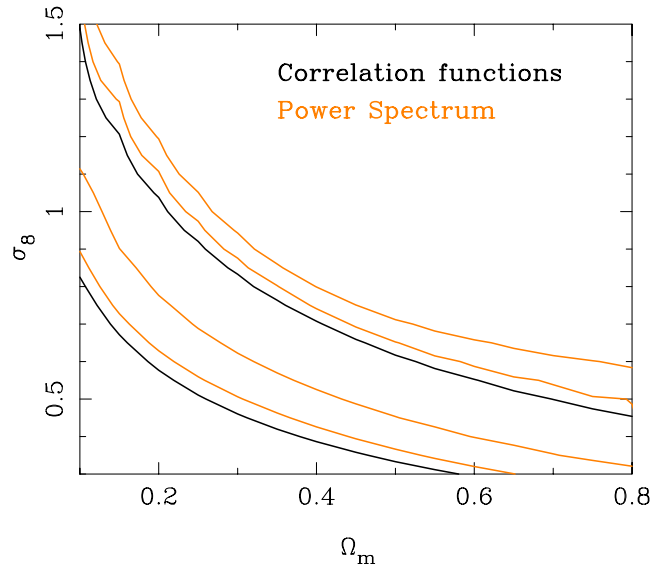
Figure 14. The likelihood surface of \sigma_8 and \Omega_m from GEMS as calculated using the shear correlation function (dark contour) and using the shear power spectrum (light contours). We plot the 1\sigma and 2\sigma confidence regions for the shear power spectrum, and, for clarity, the 1\sigma confidence regions for the shear correlation function.
