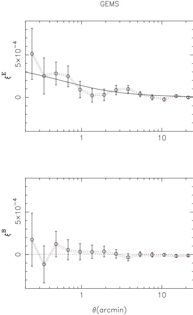
Figure 10. E/B mode decomposition of the shear correlation function measured from the GEMS observations. The upper panel shows \xi_E^{\text{bin}} and the fiducial \Lambda CDM theoretical \xi^E(\theta) model where \sigma_8 = 0.7 and the median source redshift z_m = 1.0 . The lower panel shows \xi_B^{\text{bin}} that is consistent with zero on all angular scales and can be compared to the theoretical model \xi^E(\theta) shown dotted. Using a different fiducial \Lambda CDM cosmological model to calculate \xi^{\text{bin}} has a small effect (at the level of 10^{-5} ) which can be seen from the dotted curves where we have assumed \sigma_8 = 0.6 (lower curve E-mode, upper curve B-mode) and \sigma_8 = 1.0 (upper curve E-mode, lower curve B-mode).
