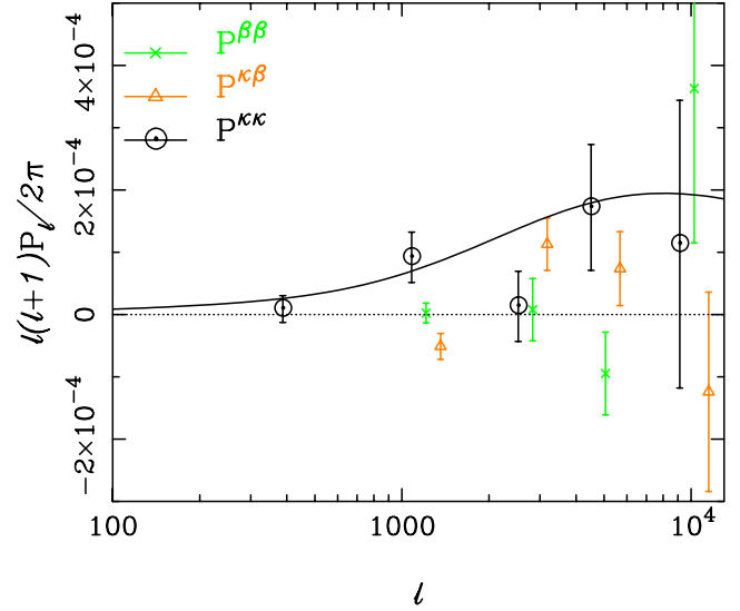
Figure 13. The cosmic shear power spectra from GEMS. Plotted on a linear-log scale are P^{\kappa\kappa} (circles), P^{\beta\beta} (crosses) and P^{\kappa\beta} (triangles) in five band-averaged band-powers as a function of multipole, l . The errors bars are estimated from the Fisher matrix and the P^{\beta\beta} and P^{\kappa\beta} have been slightly horizontally displaced for clarity. The solid curve is the shear power spectrum estimated for a \sigma_8 = 0.8 normalized \Lambda CDM model.
