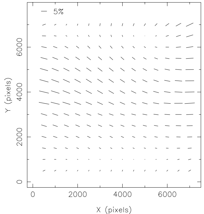
Figure 6. The difference between stellar ellipticity calculated from PSF models for each of the two GEMS data sets with r_g = 5.9 pixel. This shows that PSF variation is not a simple change in average ellipticity but also an instability in the PSF anisotropy across the field of view, varying at the maximum level of \Delta \epsilon^* = 5 per cent.
