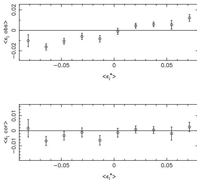
Figure 3. The upper panel shows the correlation between the mean observed galaxy ellipticity ( \epsilon_i^{\text{obs}} ) averaged in square cells of side 20 arcsec, and the cell stellar ellipticity ( \epsilon_i^* ) measured with r_g = 5.9 pixel. Correction for the anisotropic PSF removes this correlation which can be seen in the lower panel where the mean PSF corrected galaxy ellipticity ( \epsilon_i^{\text{cor}} ) is shown as a function of stellar ellipticity. Note that the upper and lower panels are plotted on different scales.
