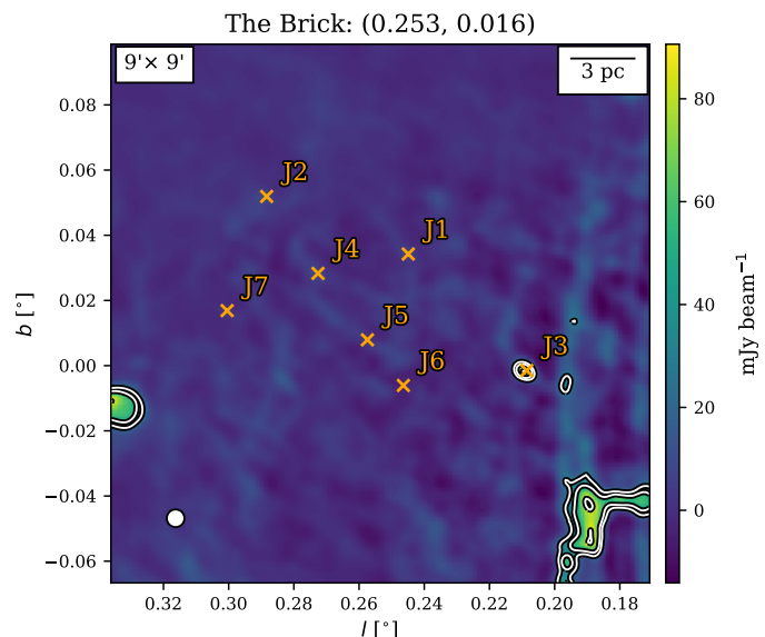
Fig. 10: GLOSTAR cutout of a 9' \times 9' area encompassing the region known as ‘the Brick’. Plotted in white contours are 3, 5, and 10 times the local rms ( 8 \text{ mJy beam}^{-1} ). Labeled in orange are the positions and names of the seven radio sources found by Rodríguez & Zapata (2013) using the VLA B- and C-configuration.
