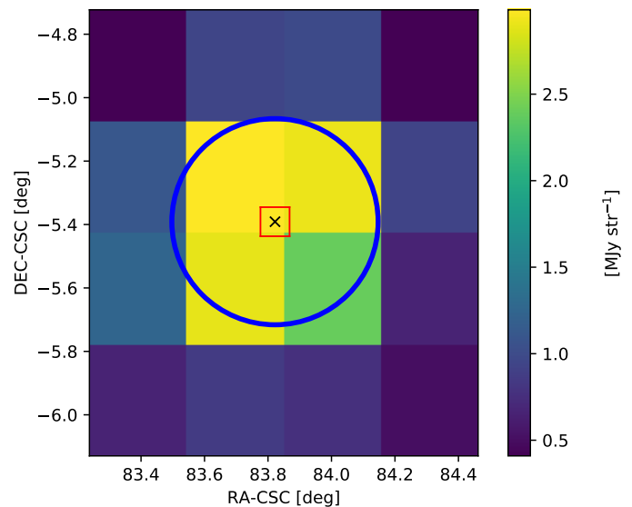
Fig. 2: COBE 2.2 \mu\text{m} data of the ONC plotted in equatorial coordinates (CSC; COBE quadrilateralised spherical cube projection). The x marker denotes the position of the ONC with the surrounding red square signifying a 5' width, which is the estimated angular size of the ONC. The size of a DIRBE pixel is 0.32^\circ . The blue circle highlights the four pixels selected for the flux determination.
