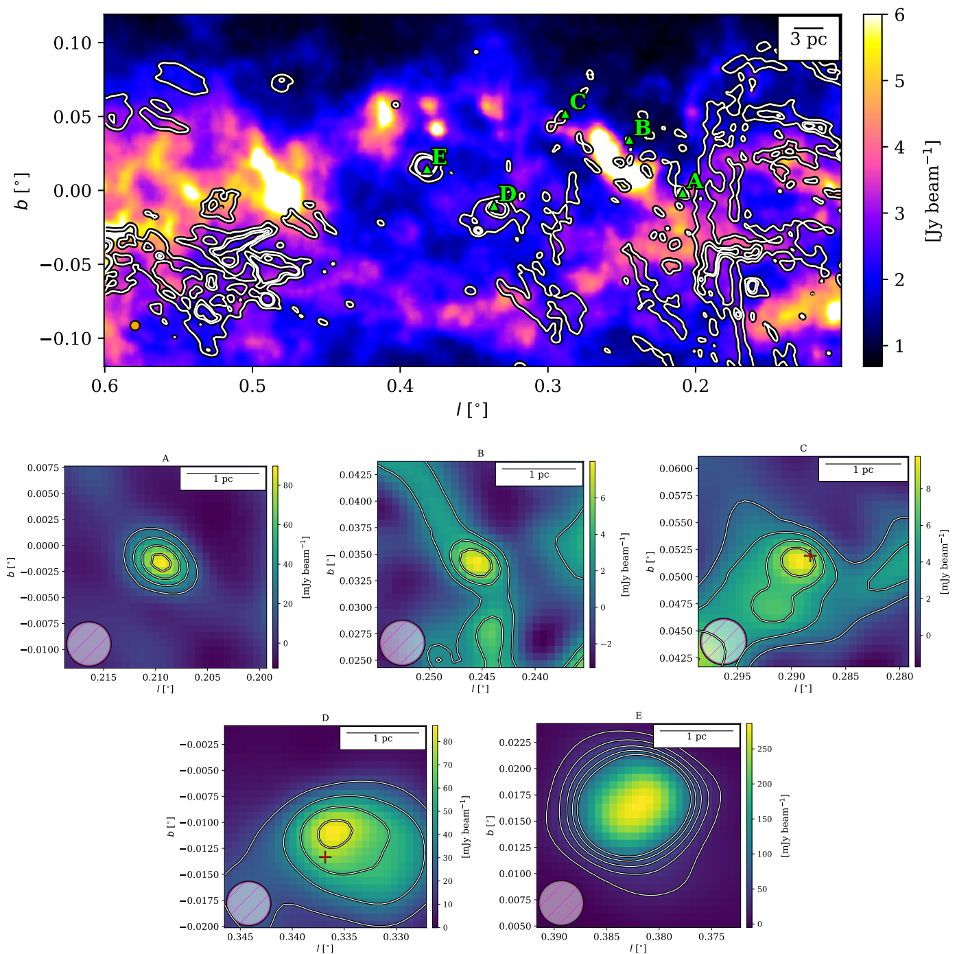
Fig. 8: Maps of the dust ridge presented similar to Fig. 5 in Immer et al. (2012a). Top : ATLASGAL 870\ \mu\text{m} dust emission towards the dust ridge with GLOSTAR 5.8 GHz radio continuum contours overlaid with contour levels of 2%, 8%, and 13% of the maximum. Bottom : GLOSTAR VLA cutouts of sources A-E cut to a larger angular size compared to Immer et al. (2012a). For sources A, D, and E, the contours are from 10\sigma to 50\sigma in steps of 10\sigma . For sources B and C, the contour levels are 4\sigma , 12\sigma , and 20\sigma . Red crosses denote the positions of YSOs.
