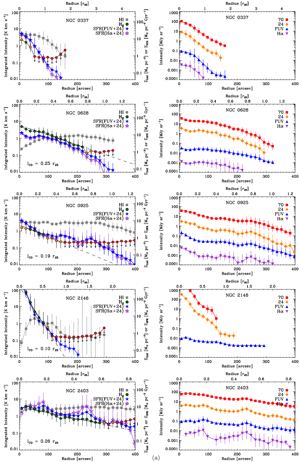
Figure A1. Atlas of radial profiles, see Figure 4 for details.
