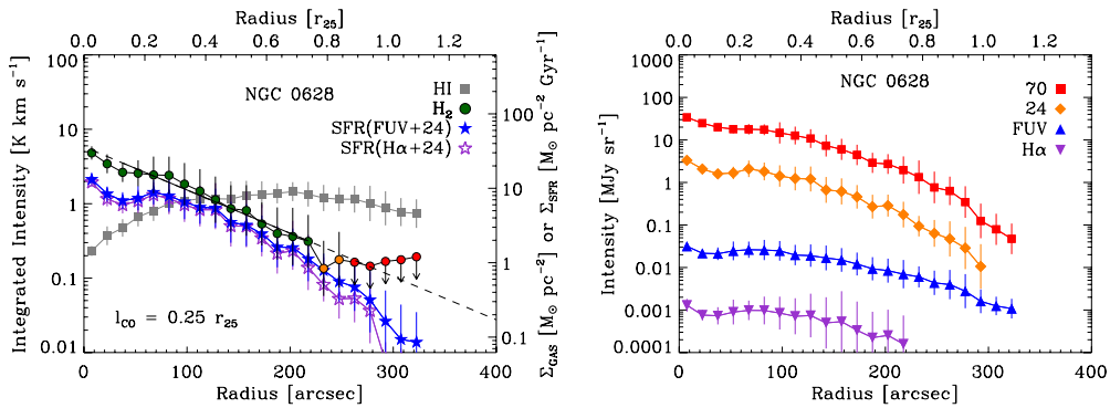
Figure 4. Azimuthally averaged intensity in 15'' wide tilted rings in NGC 628: left: H I, H 2 , and SFR from FUV + 24 \mu\text{m} and H \alpha + 24 \mu\text{m} ; right: 24 \mu\text{m} , 70 \mu\text{m} , FUV, and H \alpha intensity. Left-hand y-axes show observed intensities, the right-hand y-axis shows the surface densities of H I, H 2 , and SFR projected to face-on values. The color of the CO points indicates the significance of the fit to the stacked spectrum: high quality in green, marginal quality in orange, and upper limits in red. The solid dashed line shows an exponential fit to the radial CO profile with the scale length, l_{\text{CO}} , printed in the lower left corner. Error bars show the 1\sigma scatter inside each tilted ring. Note that we have scaled the H I intensities (left y-axis) by a factor of 312.5 in order to match all profiles in units of surface density (see text).
