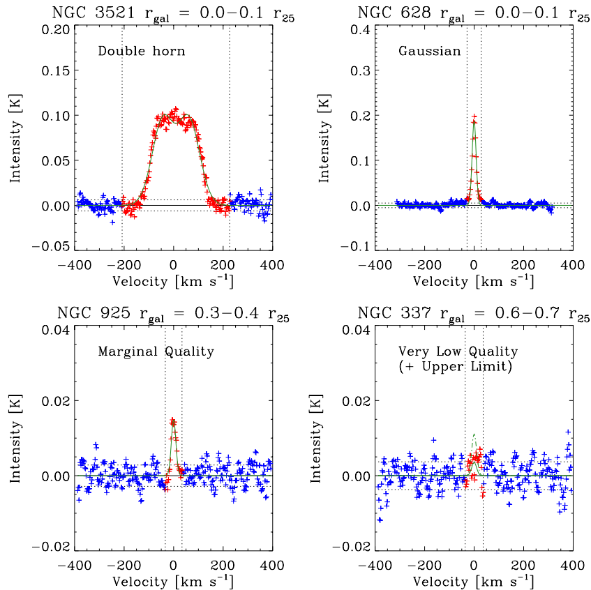
Figure 3. Examples of stacked CO spectra with different line shapes. The upper row shows spectra with high quality fits and the lower row shows spectra with low quality fits. The horizontal dotted lines mark the 1\sigma rms noise of the stacked spectrum. The upper left panel shows a broad line approximated by a double-horn profile. The upper right panel shows a narrow line fitted by a Gaussian. The lower left panel shows a marginal quality fit. The lower right panel shows a low quality fit together with the associated upper limit (dashed line).
