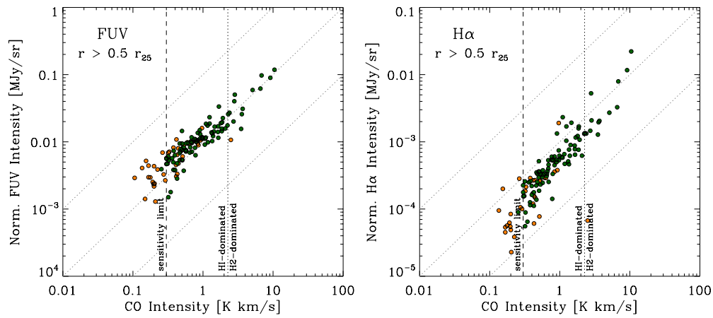
Figure 7. Relation between CO intensity and normalized FUV intensity (left panel) and normalized H \alpha intensity (right panel) for outer disks, r > 0.5 r_{25} . For each galaxy we use power-law fits to the data of high quality and normalize the relation by the FUV or H \alpha intensity, respectively, which the fit has at 1 \text{ K km s}^{-1} . (A color version of this figure is available in the online journal.)
