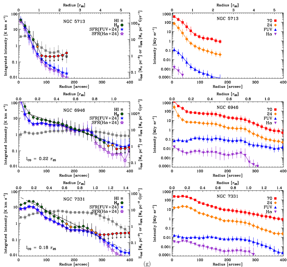
Figure A1. (Continued)
