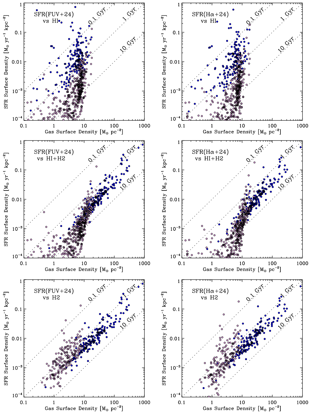
Figure 11. \Sigma_{\text{SFR}} (y-axis) from FUV + 24 \mu\text{m} (left) and \text{H}\alpha + 24 \mu\text{m} (right) as a function of different gas phases: H I alone (top), H I+H 2 (middle), and H 2 alone (bottom). Each point in these diagrams represents a radial average in a given galaxy. Regions that are H 2 -dominated are plotted with dark blue symbols, regions that are H I-dominated in light red symbols. The bottom panels show only regions with at least marginal CO signal, while the top and middle panels show also regions where we determined only an upper limit on the molecular content. Whereas SFR is not correlated with H I (in the inner parts of galaxy disks), it correlates with H 2 and total gas. The scaling with H 2 is uniform and linear for all regimes; the scaling with total gas exhibits a change in slope at the transition between H I- and H 2 -dominated environments.
