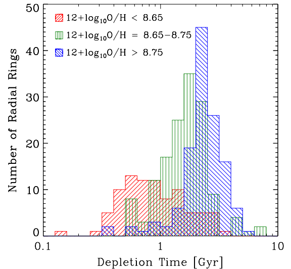
Figure 10. Molecular gas depletion time, \tau_{\text{dep}} = \Sigma_{\text{H}_2} / \Sigma_{\text{SFR}} , as a function of metallicity. The depletion times shown here correspond to the ratio of the data shown in Figure 8 including regions with CO measurements of marginal significance. The median average \tau_{\text{dep}} changes systematically with metallicity: for the low-metallicity bin \sim 0.8 Gyr, for the intermediate-metallicity bin \sim 1.7 Gyr, and for the high-metallicity bin \sim 2.4 Gyr.
