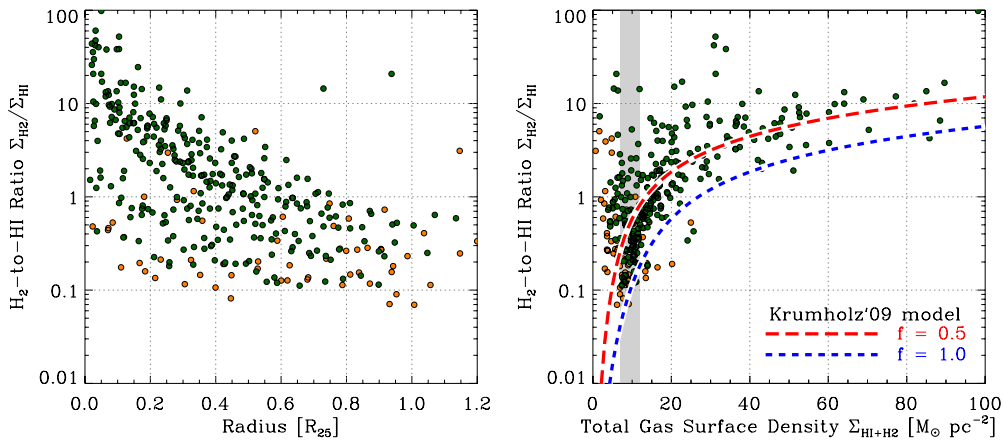
Figure 13. Molecular–atomic ratio, R_{\text{H}_2} = \Sigma_{\text{H}_2}/\Sigma_{\text{HI}} as a function of galactocentric radius (left panel), and total gas surface density, \Sigma_{\text{HI}+\text{H}_2} (right panel). The dotted line in the right panel shows R_{\text{H}_2} as predicted by a theoretical model by Krumholz et al. (2009, see text). The gray shaded area indicates data that are shown as a function of radius in Figure 14. We observe large variations in R_{\text{H}_2} as a function of radius and total gas surface density, however neither quantity is sufficient to parameterize the observed trend.
