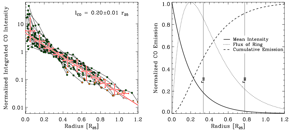
Figure 12. Left: normalized CO intensity (y-axis) as a function of galactocentric radius (x-axis) in units of r_{25} , the 25th magnitude B -band isophote for a respective galaxy. The CO intensity is normalized so that an exponential fit to the profile has intensity 1 at 0.3 r_{25} . Crosses mark the median and the 1\sigma scatter among galaxies in a series of radial bins (including only galaxies with at least marginal data in that bin). The average decline can be parameterized by an exponential with scale length of 0.2 r_{25} with no clear evidence of a truncation or break. Right: schematic diagram for an exponential disk with scale length 0.2 r_{25} . We plot mean intensity, flux in each ring, and enclosed luminosity as functions of radius. Gray lines show r_{50} and r_{90} , the radii at which 50% and 90% of the flux are enclosed.
