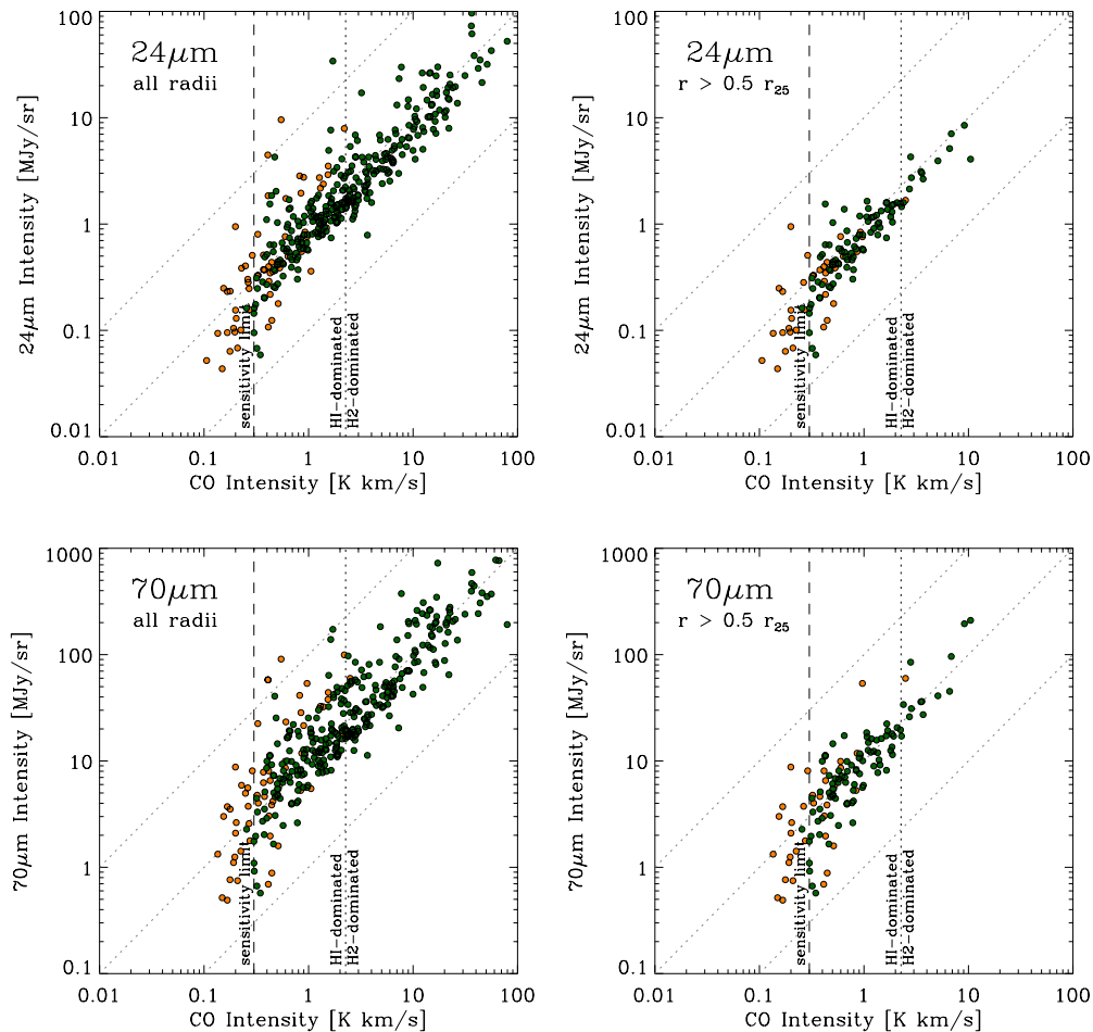
Figure 5. Observed IR intensities (y-axis) as a function of integrated CO(2 \rightarrow 1) intensity (x-axis). Each point corresponds to a stacked average in a tilted ring 15'' wide. Green and orange symbols indicate CO measurements of high or marginally significance; radial rings with only upper limits on the CO intensity (not shown here) are located exclusively to the left of the long-dashed line. The top panels show the relation of 24 \mu\text{m} vs. CO, the bottom panels shows 70 \mu\text{m} vs. CO. The left panels show data for all radii, whereas the right panels show only data outside 0.5r_{25} , where the ISM is typically H I-dominated. The short-dashed vertical line indicates a typical CO intensity at which \Sigma_{\text{H}_2} \sim \Sigma_{\text{H I}} ; data to the left of this line will usually be H I-dominated. The diagonal dashed lines indicate lines of constant ratios for orientation.
