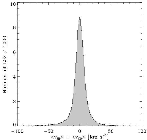
Figure 1. Difference between local mean velocities of H I and CO for lines of sight with galactocentric radius smaller than 0.5 r_{25} . The close correspondence motivates our use of the H I mean velocity to predict the CO velocities in low surface brightness regions.
