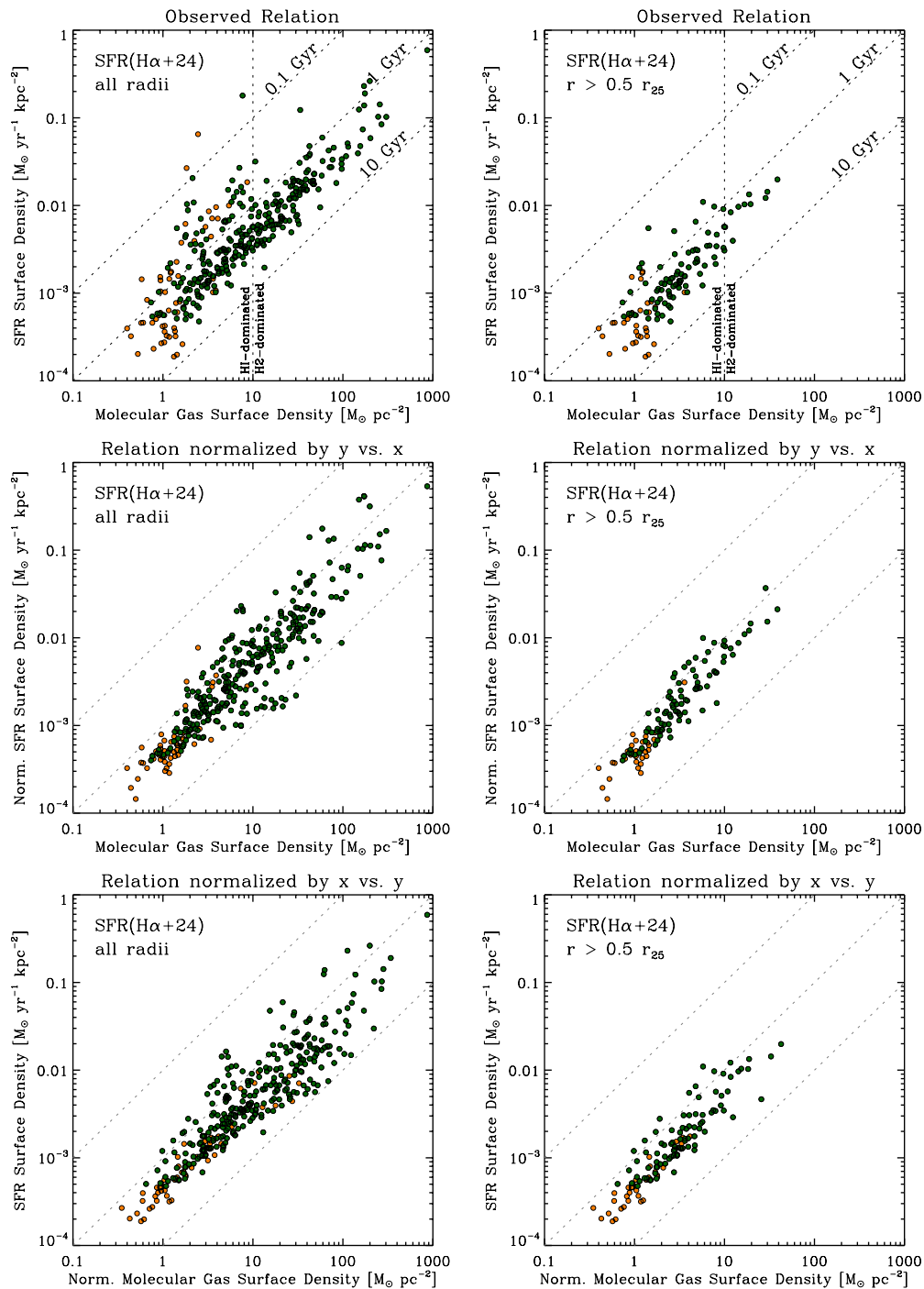
Figure 9. Same plot as Figure 8 but this time using H\alpha + 24\ \mu\text{m} to estimate \Sigma_{\text{SFR}} . (A color version of this figure is available in the online journal.)
