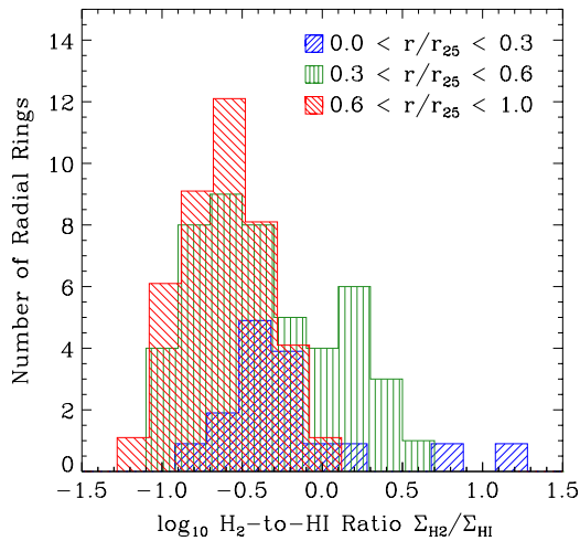
Figure 14. Radial dependence of R_{H_2} for regions with comparable total gas surface density, \Sigma_{H_1+H_2} = 7\text{--}12 M_{\odot} \text{pc}^{-2} . The data are taken from the gray highlighted region in the left panel of Figure 13. R_{H_2} is not sufficiently determined by the total gas surface density but shows also a radial dependence. (A color version of this figure is available in the online journal.)
