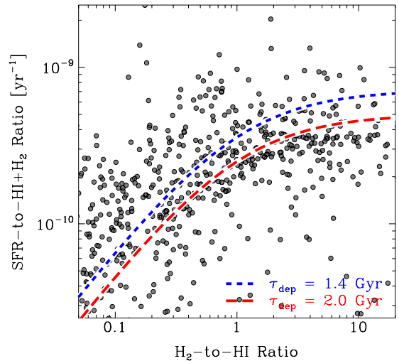
Figure 15. Recent star formation rate per unit total gas, \Sigma_{\text{SFR}}/\Sigma_{H_1+H_2} (the inverse of the total gas depletion time; y-axis), as a function of the molecular–atomic gas ratio, R_{H_2} = \Sigma_{H_2}/\Sigma_{H_1} (x-axis). A fixed ratio of SFR-to- H_2 is shown by the blue dotted line for a molecular gas depletion time of \tau_{\text{dep}} \approx 1.4 Gyr and by the red dashed line for \tau_{\text{dep}} \approx 2.0 Gyr. In regions dominated by molecular gas ( R_{H_2} > 1 ) the \Sigma_{\text{SFR}}/\Sigma_{H_1+H_2} ratio approximates a value corresponding to the constant molecular depletion time, \tau_{\text{dep}} . In regions of small molecular gas fraction ( R_{H_2} < 1 ) the \Sigma_{\text{SFR}}/\Sigma_{H_1+H_2} ratio decreases significantly indicating that the total gas does not scale uniformly with the recent star formation rate. (A color version of this figure is available in the online journal.)
