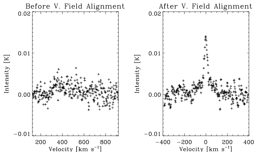
Figure 2. Average CO spectrum across tilted ring spanning from 0.7 to 0.8 r_{25} in NGC 5055. The left panel shows the result of a simple average of all spectra. The right panel shows that the average after each spectrum is shifted so that v = 0 corresponds to the local mean H I velocity.
