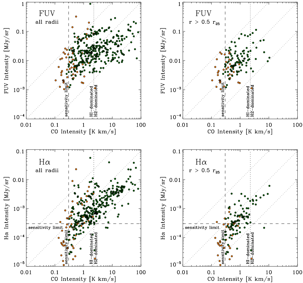
Figure 6. Similar plot as Figure 5 but this time showing the relation of FUV vs. CO and H \alpha vs. CO for our two radial ranges. Note that H \alpha intensities below a few times 10^{-4} MJy sr ^{-1} are affected by data quality and processing and have to be considered uncertain.
