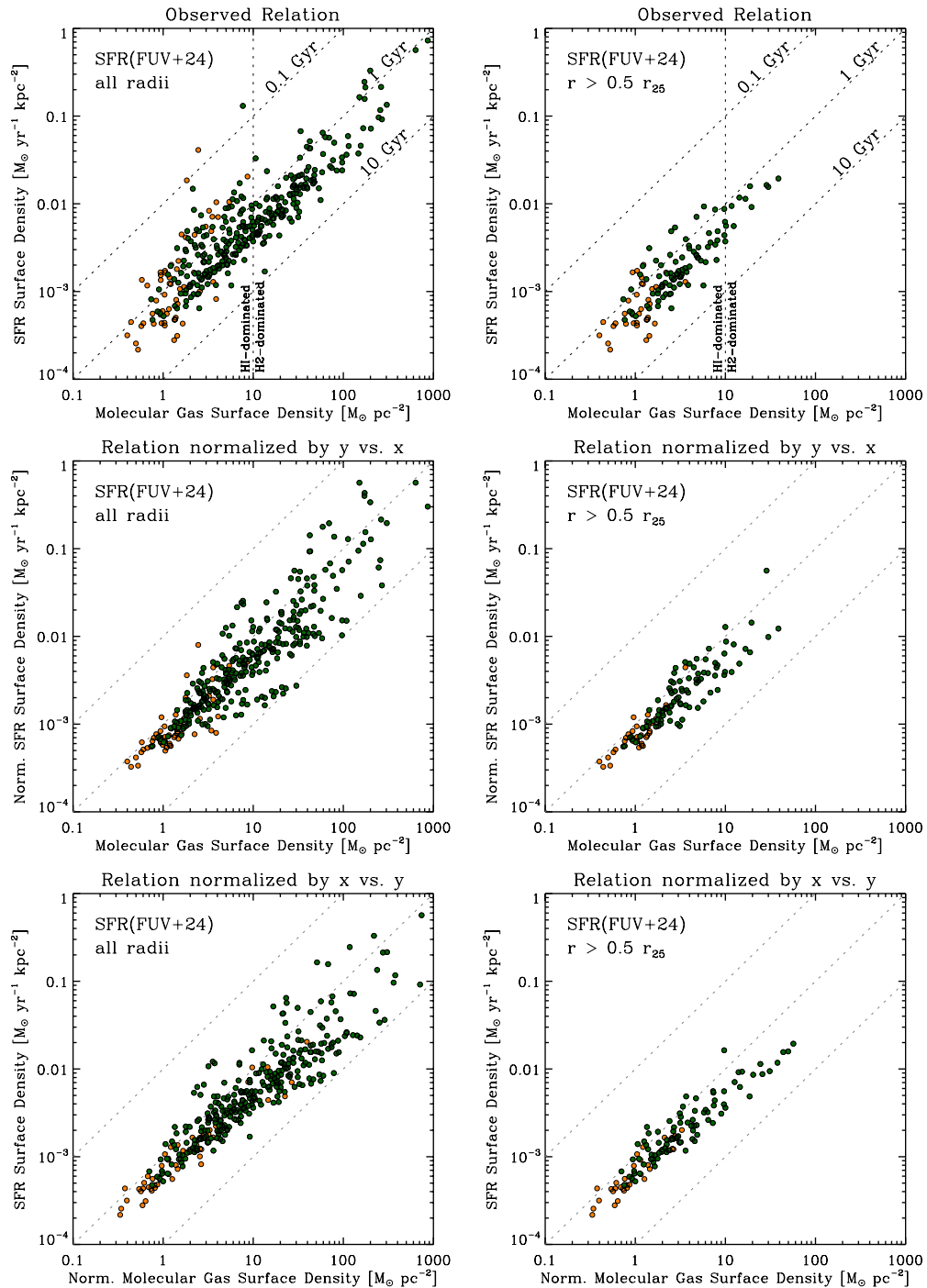
Figure 8. Recent star formation rate surface density estimate from FUV + 24 \mu\text{m} ( y -axis) as a function of molecular gas surface density ( x -axis). The left-hand column shows data for all radii, whereas the right-hand column shows only data where r > 0.5r_{25} . The upper row presents the basic relation, which is approximately linear with average \text{H}_2 depletion time \sim 2.0 Gyr (dashed lines). The middle and bottom rows show results after we fit and remove galaxy-to-galaxy variations. These galaxy-to-galaxy variations are \sim 2 times larger than internal variations, suggesting individual galaxies each obey well-defined, though offset, relations.
