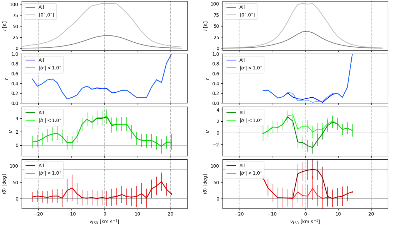
Fig. 17: Synthetic H \alpha emission intensity and circular statistics used for the study of the orientation of the H \alpha filamentary structures across velocity channels in the synthetic observations presented in Fig. 16. Top . H \alpha emission averaged over the whole map and toward the indicated position. Middle top . Mean resulting vector ( r ), which indicates if the distribution of orientation angles is flat ( r \approx 0 ) or sharply unimodal ( r \approx 1 ). Middle bottom . Projected Rayleigh statistic ( V ), which indicates if the distribution of orientation angles is clearly peaked around 0^\circ ( V \gg 0 ) or 90^\circ ( V \ll 0 ). Bottom . Mean orientation angle ( \langle \theta \rangle ) of the H \alpha filamentary structures.
