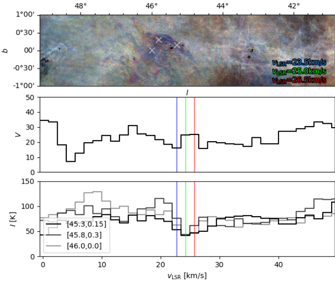
Fig. 13: Selected example of a prominent HI self-absorption (HISA) structure. Top . Atomic hydrogen (HI) emission in three velocity channels. Middle . Projected Rayleigh statistic ( V , Eq. 5) corresponding to the orientation of the filamentary structures in the HI emission in the corresponding channels. Bottom . Spectra toward the positions indicated by the crosses in the top panel. The vertical lines indicate the v_{\text{LSR}} that corresponds to the emission shown in the other two panels.
