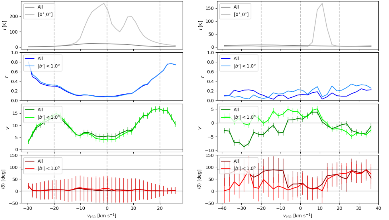
Fig. 19: Synthetic H \alpha emission intensity and circular statistics used for the study of the orientation of the H \alpha filamentary structures across velocity channels in the synthetic observations presented in Fig. 18. Top . H \alpha emission averaged over the whole map and toward the indicated position. Middle top . Mean resulting vector ( r ), which indicates if the distribution of orientation angles is flat ( r \approx 0 ) or sharply unimodal ( r \approx 1 ). Middle bottom . Projected Rayleigh statistic ( V ), which indicates if the distribution of orientation angles is clearly peaked around 0^\circ ( V \gg 0 ) or 90^\circ ( V \ll 0 ). Bottom . Mean orientation angle ( \langle \theta \rangle ) of the H \alpha filamentary structures.
