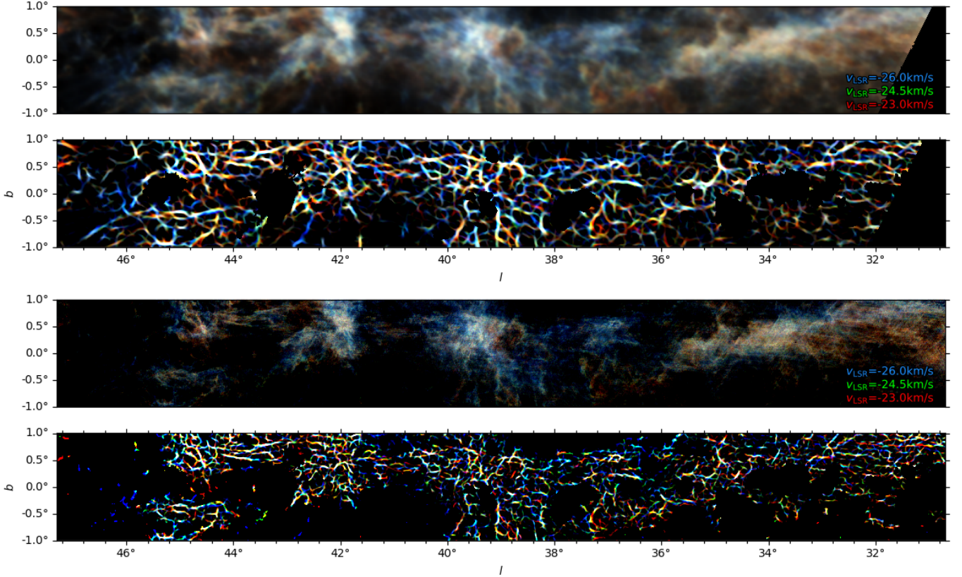
Fig. 5: GALFA-H I (top) and THOR-H I (bottom) observations and their respective filaments from the Hesssian analysis toward the same region of the Galactic plane in the indicated velocity channels.
