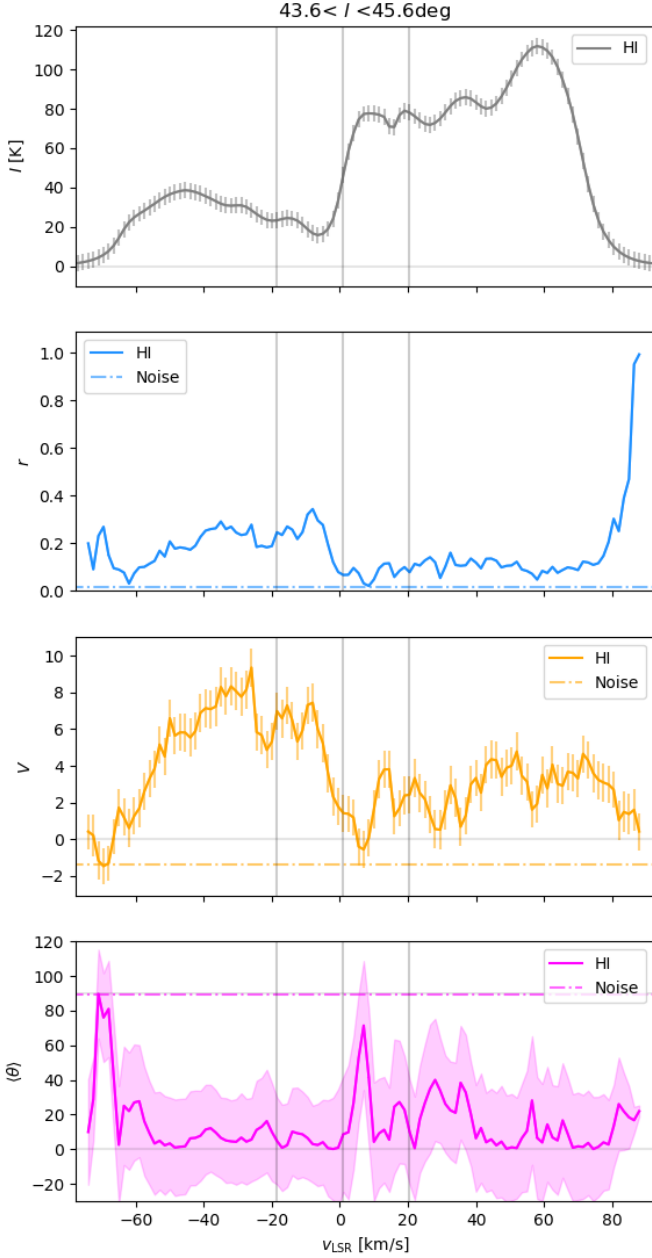
Fig. 3: Mean spectrum and circular statistics used for the study of the orientation of the H I filamentary structures across velocity channels toward the region presented in Fig. 1. Top. Mean H I intensity ( I ). Middle top. Mean resulting vector ( r ), which indicates if the distribution of orientation angles is flat ( r \approx 0 ) or sharply unimodal ( r \approx 1 ). Middle bottom. Projected Rayleigh statistic ( V ), which indicates if the distribution of orientation angles is clearly peaked around 0^\circ ( V \gg 0 ) or 90^\circ ( V \ll 0 ). Bottom. Circular mean ( \langle\theta\rangle ) and standard deviation ( \sigma_V ) of the orientation angles, represented by the line and the shaded area, respectively. The error bars correspond to the observation uncertainties and the error propagation based on the Monte Carlo sampling introduced in App. A.1. The dashed horizontal lines in each panel indicate the values of those quantities in the 1.4 GHz noise maps used to characterize the effect of the side lobes and continuum sources in the H I maps. The vertical gray lines correspond to the velocity channels shown in Fig. 1.
