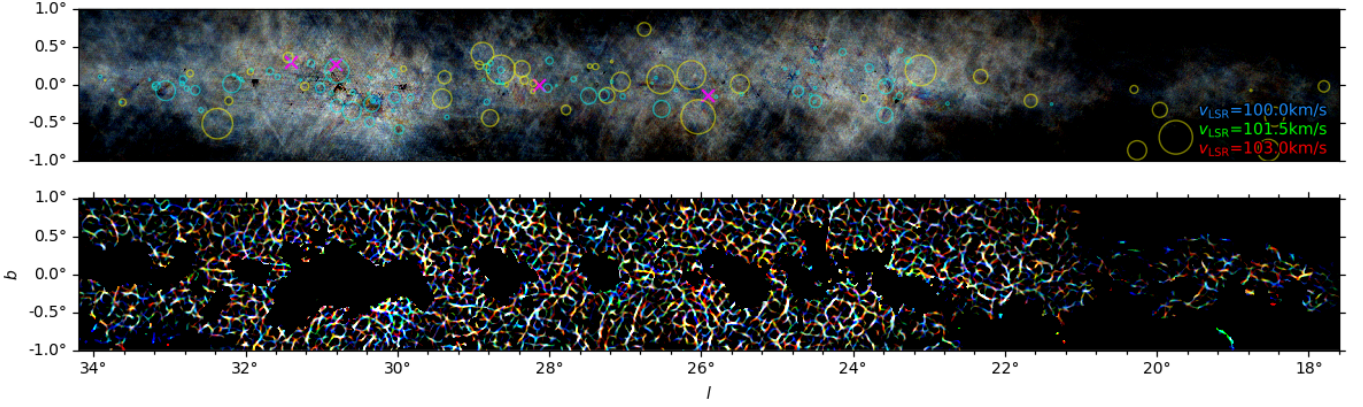
Fig. 10: THOR-H I (top) observations and their respective filaments from the Hessian analysis (bottom) toward the Galactic longitude range of the region of interest (ROI) A, as defined in Fig 7. The yellow circles correspond to the positions and sizes of the supernova remnants in the Green (2019) catalogue. The cyan circles correspond to the positions and sizes of the H II regions in the Anderson et al. (2014) catalogue with v_{\text{LSR}} within \pm 10 \text{ km s}^{-1} of the central velocity indicated in the figure. The magenta crosses mark the position of the THOR OH 1720-MHz masers in that velocity range.
