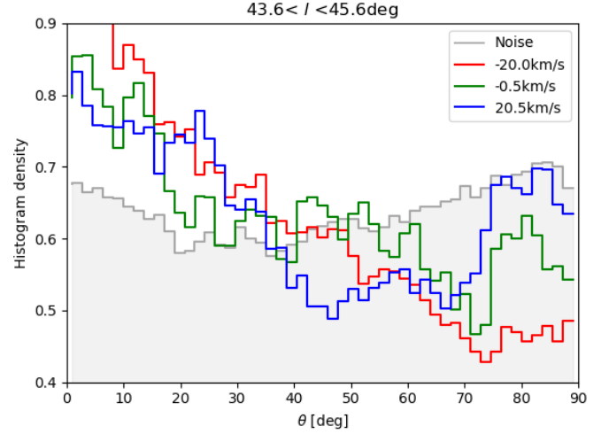
Fig. 2: Histograms of orientation angles ( \theta , as defined in Eq. 3) of the filamentary structures obtained by applying the Hessian matrix method to the velocity channels maps presented in Fig. 1. The angles \theta = 0^\circ and \theta = 90^\circ correspond to the directions parallel and perpendicular to the Galactic plane, respectively.
