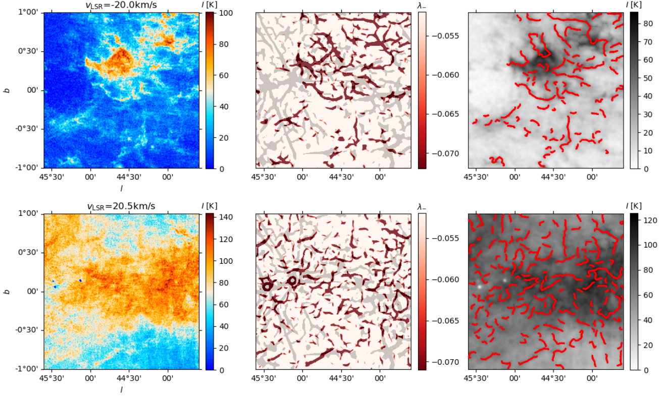
Fig. C.1: Example of the FilFinder application to a pair of velocity channel maps in THOR-H I . Left. Intensity map at the indicated line-of-sight velocity. Middle. Map of the eigenvalue \lambda_- obtained with a 120' FWHM derivative kernel. This map is used as a mask for FilFinder. Right. FilFinder filaments overlaid on the respective H I intensity map smoothed to 120' FWHM.
