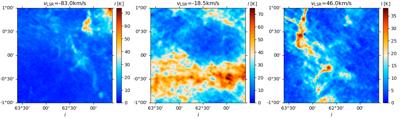
Fig. 14: THOR-H \alpha emission for two velocity channels in the region of interest (ROI) D (left and right) and a channel toward the same l range but dominated by filaments parallel to the Galactic plane (middle).
