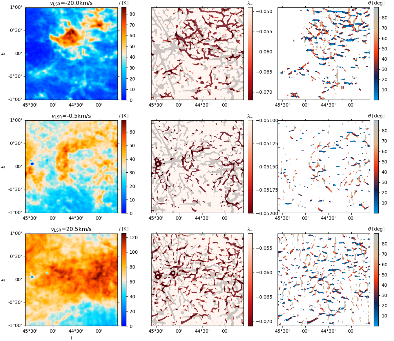
Fig. 1: Examples of the Hessian analysis applied to three different velocity-channel maps toward a section of the Galactic plane observed by THOR. Left . Intensity map. Center . Map of the eigenvalue of the Hessian matrix identified as \lambda_- in Eq. (2), which is used to characterize the filamentary structures in the intensity map. The overlaid grey map shows the filamentary structure obtained from the Hessian matrix analysis of the continuum noise maps, see App. A for details. Right . Map of the orientation angles evaluated using Eq. (3).
