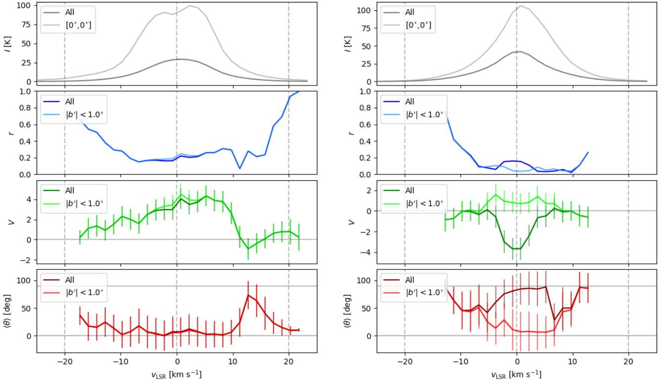
Fig. D.2: Synthetic H I emission intensity and circular statistics used for the study of the orientation of the H I filamentary structures across velocity channels in the synthetic observations presented in Fig. D.1. Top . H I emission averaged over the whole map and toward the indicated position. Middle top . Mean resulting vector ( r ), which indicates if the distribution of orientation angles is flat ( r \approx 0 ) or sharply unimodal ( r \approx 1 ). Middle bottom . Projected Rayleigh statistic ( V ), which indicates if the distribution of orientation angles is clearly peaked around 0^\circ ( V \gg 0 ) or 90^\circ ( V \ll 0 ). Bottom . Mean orientation angle ( \langle\theta\rangle ) of the H I filamentary structures.
