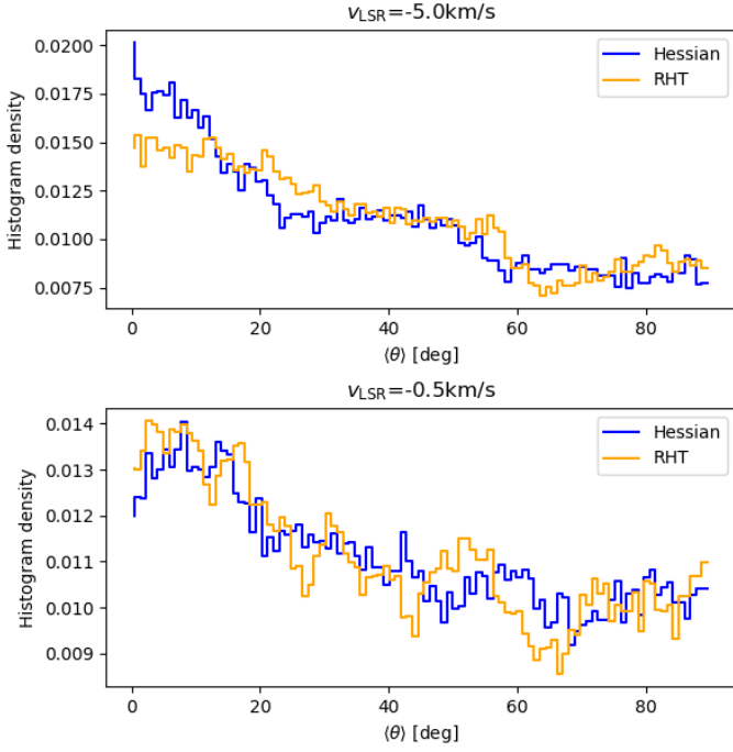
Fig. C.3: Histograms of the orientation of the filamentary structures identified using the Hessian matrix and the RHT methods in the velocity-channel maps presented in Fig. C.2.
