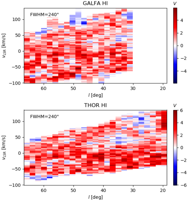
Fig. B.2: Longitude-velocity diagram of the projected Rayleigh statistic V corresponding to the results of the Hessian analysis of the GALFA-HI and THOR-HI observations, shown in the top and bottom. Both results were obtained with the same derivative kernel size, indicated in the figure.
