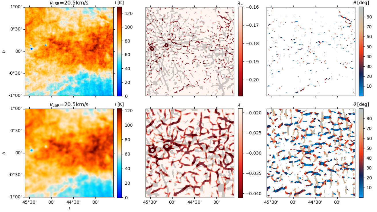
Fig. A.3: Same as Fig. 1 for derivative kernels of 80'' (top) and 160'' FWHM (bottom), which correspond to two and four times the native resolution of the THOR-H I observations, respectively.
