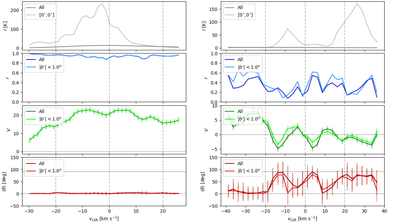
Fig. E.2: Synthetic H I emission intensity and circular statistics used for the study of the orientation of the H I filamentary structures across velocity channels in the synthetic observations presented in Fig. E.1. Top . H I emission averaged over the whole map and toward the indicated position. Middle top . Mean resulting vector ( r ), which indicates if the distribution of orientation angles is flat ( r \approx 0 ) or sharply unimodal ( r \approx 1 ). Middle bottom . Projected Rayleigh statistic ( V ), which indicates if the distribution of orientation angles is clearly peaked around 0^\circ ( V \gg 0 ) or 90^\circ ( V \ll 0 ). Bottom . Mean orientation angle ( \langle \theta \rangle ) of the H I filamentary structures.
