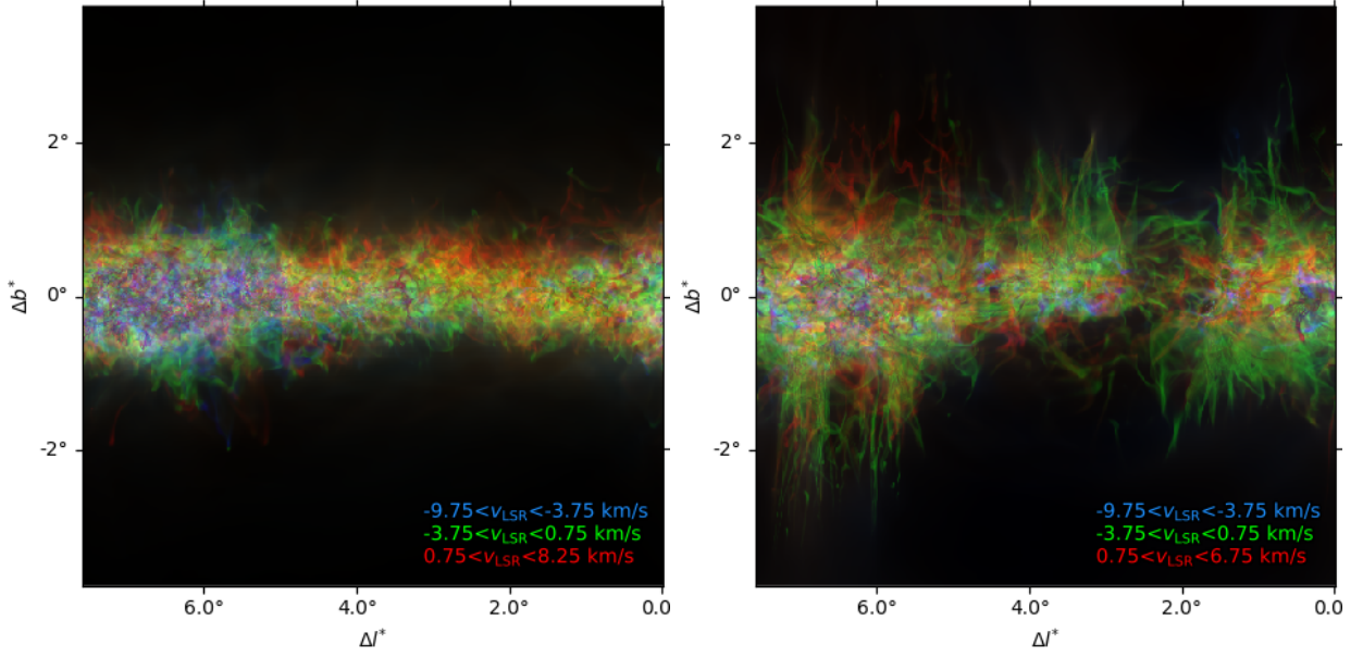
Fig. 16: Synthetic observations of the H \alpha emission from the FRIGG simulations with a standard ( 3 \mu\text{G} ) and very high ( 12 \mu\text{G} ) initial magnetizations, shown in the left and right panels, respectively. The colors represent the emission in the three indicated radial velocity bins with the same average emission.
