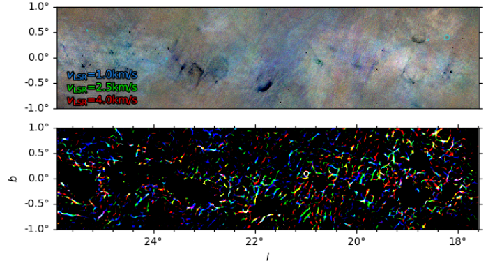
Fig. 12: Same as Fig. 10 for the ROI C.
