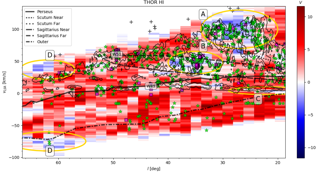
Fig. 7: Projected Rayleigh statistic ( V ) corresponding to the orientation of the filamentary structures identified with the Hessian matrix method in the H I emission in 2^\circ \times 2^\circ tiles and across velocity channels. The overlaid curves correspond to selected spiral arms from the model presented in Reid et al. (2016). The black contours corresponds to the 97 and 99 percentile of the ^{12}\text{CO} emission in the observations presented in Dame et al. (2001) integrated over the Galactic longitude range |b| \leq 1^\circ . The green stars correspond to the H II regions in the WISE catalog of Galactic H II regions (Anderson et al. 2014). The two most prominent regions of high-mass star formation in this portion of the Galaxy, W49 and W51, are indicated by the corresponding labels. The magenta crosses correspond to the 1720-MHz OH masers in the catalog (Beuther et al. 2019), which are typically excited by shocks. The black crosses correspond to the compact H I clouds at high forbidden velocities identified in the VGPS (Stil et al. 2006a). The ellipses labelled with letters indicate the regions of interest (ROIs) discussed in Sec. 5.2.
