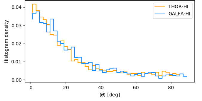
Fig. B.4: Histogram of the mean orientations of the H I filaments identified using the Hessian analysis with a 240'' FWHM derivative kernel applied to 2^\circ \times 2^\circ \times 1.5 \text{ km s}^{-1} velocity-channel tiles in the GALFA-HI and THOR-HI observations.
