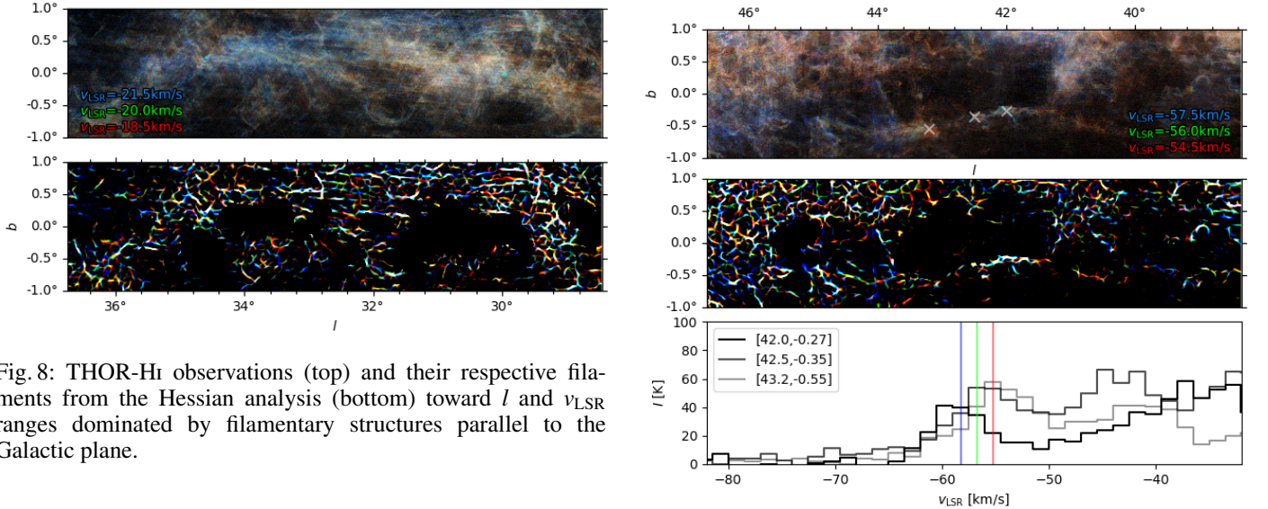
Fig. 9: Magdalena H I filament. Top . Atomic hydrogen (H I ) emission in three velocity channels. Middle . Filaments obtained using the Hessian technique toward the corresponding channels. Bottom . Spectra toward the positions indicated by the crosses in the top panel. The vertical lines indicate the v_{\text{LSR}} that corresponds to the emission shown in the other two panels.
