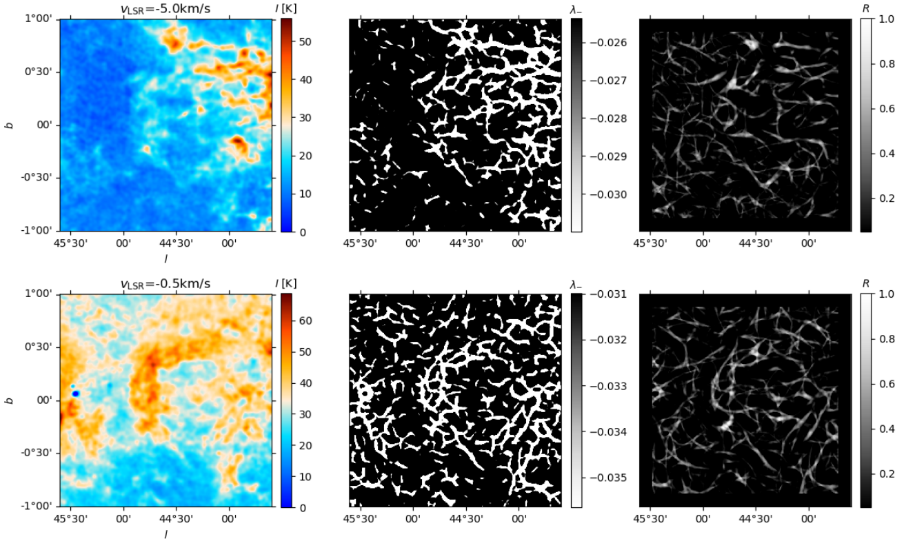
Fig. C.2: Comparison of the results of the Hessian and the RHT methods for two different velocity-channel maps toward a region within the area covered by THOR-H I . Left. Intensity map at the indicated line-of-sight velocity, v_{\text{LSR}} . Middle. Map of the eigenvalue \lambda_- of the Hessian matrix. Right. Map of the RHT backprojection.
