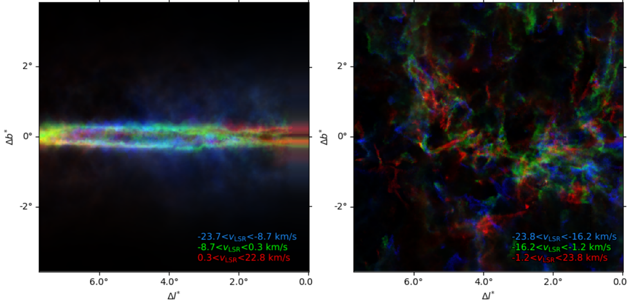
Fig. 18: Synthetic observations of the H \alpha emission from the potential and feedback dominated CloudFactory simulations, presented in the left and right panels, respectively. The colors represent the emission in the three indicated radial velocity bins, each of the with the same average emission.
