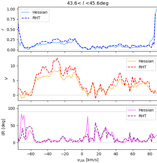
Fig. C.4: Circular statistics used for the study of the orientation of the H I filamentary structures found using the Hessian and the RHT methods across velocity channels toward the region presented in Fig. C.2. Top . Mean resulting vector ( r ), which indicates if the distribution of orientation angles is flat ( r \approx 0 ) or sharply unimodal ( r \approx 1 ). Middle . Projected Rayleigh statistic ( V ), which indicates if the distribution of orientation angles is clearly peaked around 0^\circ ( V \gg 0 ) or 90^\circ ( V \ll 0 ). Bottom . Mean orientation angle ( \langle \theta \rangle ) of the H I filamentary structures.
