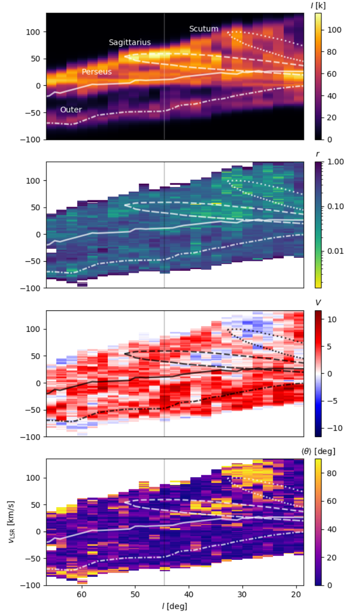
Fig. 4: Longitude-velocity ( lv ) diagrams corresponding to the mean intensity and the results of the Hessian analysis of the velocity-channel maps in the region covered by the THOR observations. Each pixel in the diagrams represents the quantities calculated in 2^\circ \times 2^\circ tile in a 1.5 \text{ km s}^{-1} -velocity channel as follows. Top. Mean H I intensity ( I ). Middle top. Mean resulting vector ( r ). Middle bottom. Projected Rayleigh statistic ( V ). Bottom. Mean orientation angle ( \langle\theta\rangle ) of the H I filamentary structures, which is only well-defined if r > 0 . The overlaid curves correspond to selected spiral arms from the model presented in Reid et al. (2016). The vertical line indicates the central l of the 2^\circ \times 2^\circ tile presented in Fig. 1 and whose circular statistics are shown in Fig. 3.
