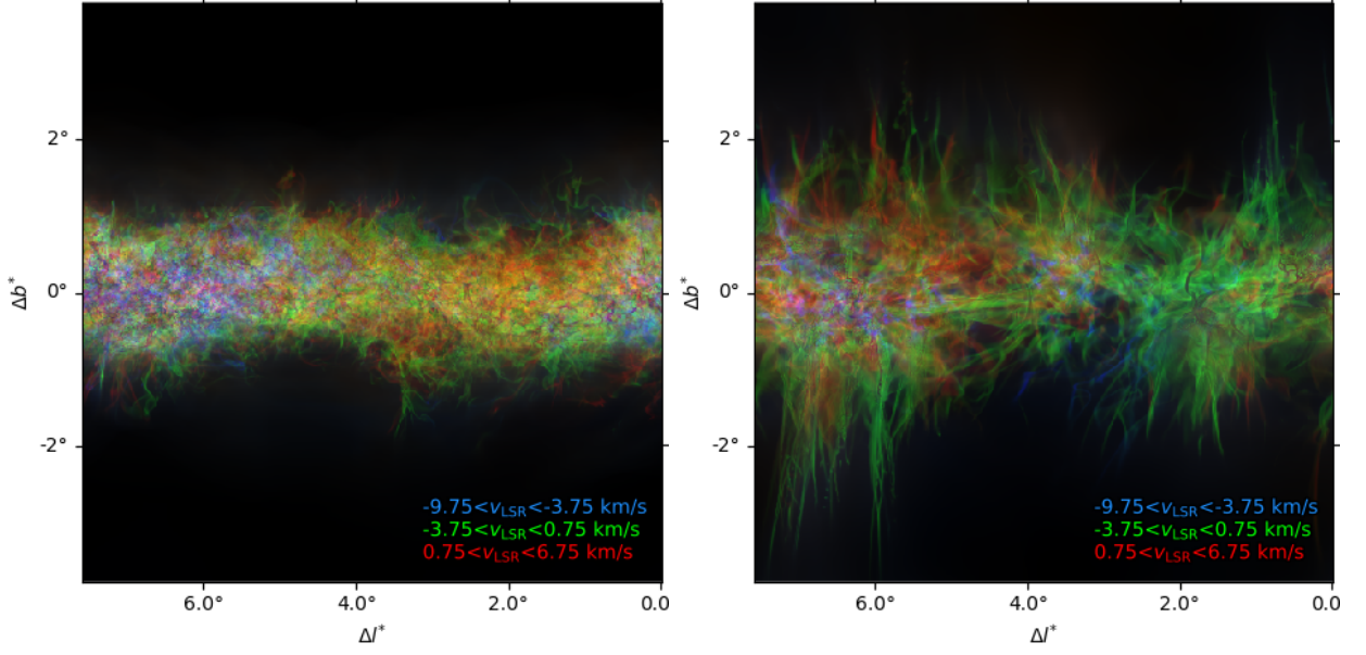
Fig. D.1: Synthetic observations of the H I emission from the FRIGG simulations with a standard ( 3 \mu\text{G} ) and very high ( 12 \mu\text{G} ) initial magnetizations, shown in the left and right panels, respectively. These snapshots are taken 14 Myr before those shown in Fig. 16. The colors represent the emission in the three indicated radial velocity bins with the same average emission.
