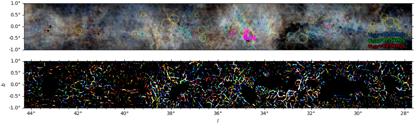
Fig. 11: Same as Fig. 10 for the ROI B.
