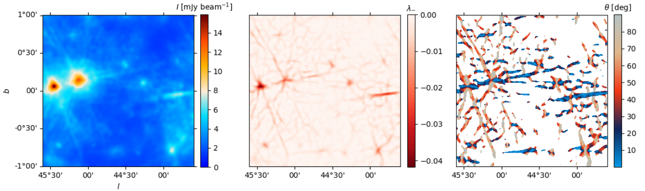
Fig. A.2: Same as Fig. A.1 for the noise map of the continuum emission at 1.42 GHz ( \sigma_{1.42} ), which we use as a proxy of the structure introduced by the side-lobes in the imaging of the H I emission.
