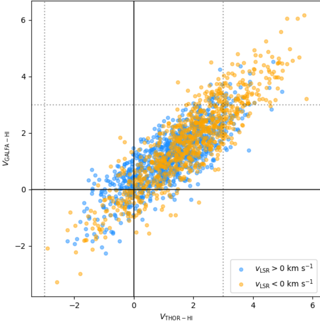
Fig. B.3: Projected Rayleigh statistic V calculated from the Hessian analysis of the GALFA-HI and THOR-HI observations using a 240'' FWHM derivative kernel. Each point corresponds to a 2^\circ \times 2^\circ \times 1.5 \text{ km s}^{-1} velocity-channel tile fully covered by both surveys. The vertical and horizontal dotted lines indicate |V| = 3 , which roughly corresponds to a 3\text{-}\sigma confidence level in the estimation of a preferential orientation of 0^\circ or 90^\circ .
