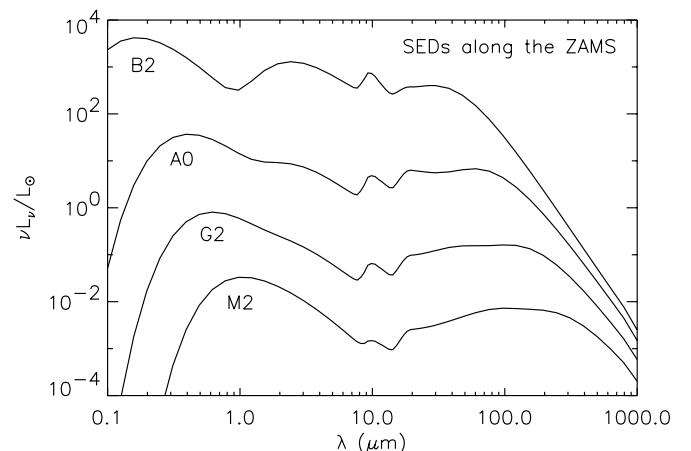
FIG. 6.—Model-predicted SED for ZAMS stars of different spectral type. The stellar parameters are given in Table 1.
