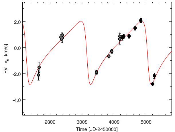
Fig. 1. RV measurements of Cha H \alpha 8 between 2000 and 2010 based on UVES/VLT spectra. New RV data measured between Jun 2007 and Mar 2010 are marked with black-filled points, previously obtained RV data with grey-filled points. Overplotted is the best-fit Keplerian orbit, which has a semi-amplitude of 2.4 km s ^{-1} , a period of 5.2 years and an eccentricity of e=0.59 .
