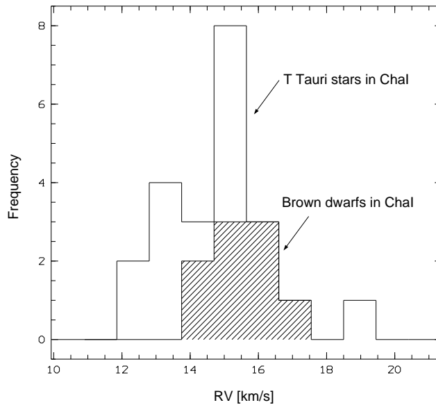
Figure 3.2: Distribution of mean radial velocities for nine bona fide and candidate brown dwarfs (hashed) and for 22 T Tauri stars in Cha I.
