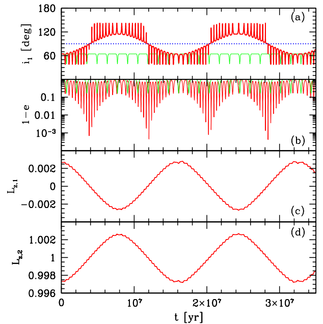
Fig. 6.— Inclination flipping due to the Lidov-Kozai mechanism when the disturbing function is truncated to octupole order (upper curve on panel a and lower curve on panel b) versus quadrupole order (lower curve on panel a and upper curve on panel b). The inner binary consists of a 1M_{\odot} star and a 1M_J planet separated by 6 au with e_{\text{in}} = 0.001 , and the outer body is a brown dwarf of 40M_J at a distance of 100 au from the center of mass of the inner binary with e_{\text{out}} = 0.6 . The bottom two plots display the normalized vertical components of the inner and outer orbit angular momentum (Figure 1 of Naoz et al. 2011 , reprinted by permission from Macmillan Publishers Ltd: Nature, 473, 187-189, copyright 2011).
