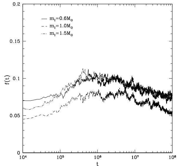
Fig. 5.— The fraction of solar systems f(t) containing planets with semi-major axes greater than 100 AU, plotted here as a function of time t after a close encounter for intruder stars of masses 0.6, 1.0 and 1.5 M_{\odot} . These simulations of fly-bys involve the four gas giants of the solar system with r_{\min} < 100 \text{ AU} (Figure 11 of Malmberg et al. 2011 , reproduced by permission of RAS).
