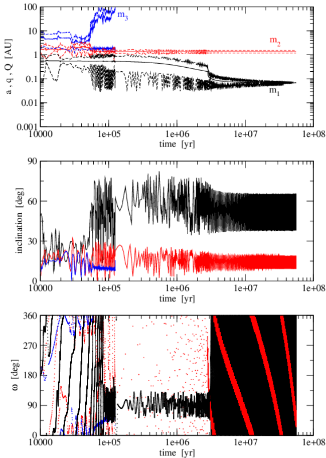
Fig. 9.— Hot Jupiter production by Lidov-Kozai forcing from multiple-planet interactions. The inner, middle and outer planets have masses of 1M_J , 2M_J and 1M_J and initially nearly circular ( e < 0.1 ) and coplanar ( I < 1^\circ ) orbits (Figure 11 of Beaugé and Nesvorný 2012 , reproduced by permission of AAS).
