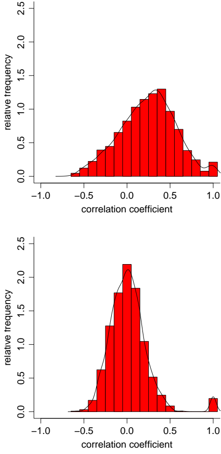
Figure 6. Histogram of the correlation coefficients for SSSPM0828 (top; from Fig. 4) and for the random spectra (bottom; from Fig. 5). The ordinate is a density (i.e. the total area is 1.0). The overlotted line is a kernel density estimate.
