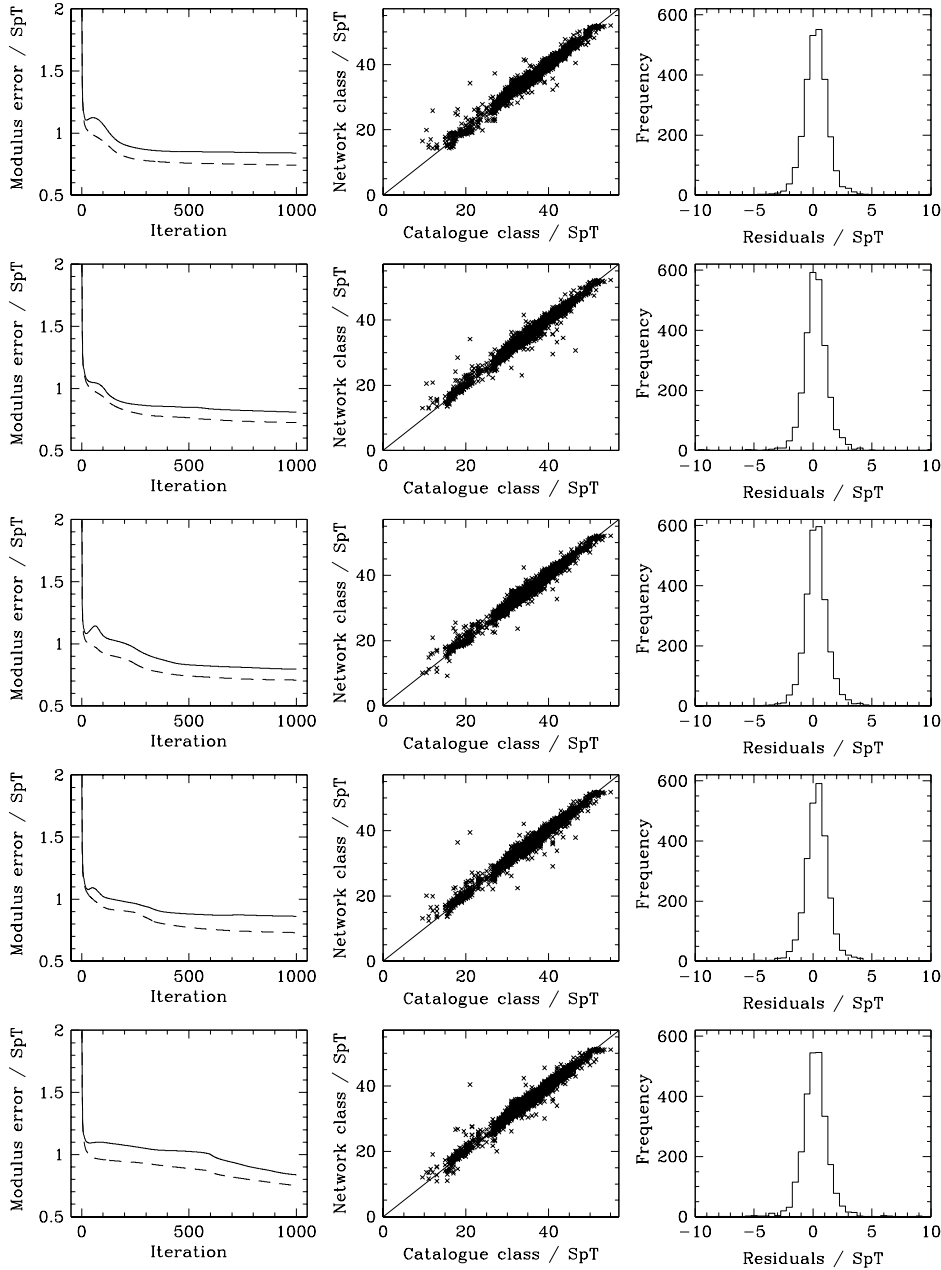
Figure 15. Performance of the first five members of the committee networks used to produce the results in Figure 14. The left-hand figures show how the neural network error drops with increasing iteration number. The dashed line shows the error on the training set and the solid line the error on the test set. Note that the network error, as measured on the test set during training, briefly increases early on in the training for the first and third networks. This demonstrates that we should not stop training the instant that the error on the test set rises. It is also interesting that most of the training takes place in the first few iterations.
