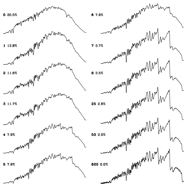
Figure 7. Reconstruction of an M star (HD 14002, type M3/4 III, magnitude 9.4). The figures in bold refer to the number of eigenvectors used to reconstruct the spectrum. The percentage figures are the corresponding reconstruction error, E . Note the improved reconstruction as the 7 th component is added.
