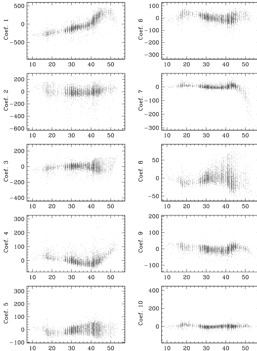
Figure 4. The first ten principal component admixture coefficients for all spectra (line+continuum format) in data set A plotted against spectral subtype (SpT). The correlation between the 7 th coefficient and spectral subtype for SpT \gtrsim 48 (M stars) is accountable by reference to Figure 3 where we see that the 7 th eigenvector gives a strong representation of the TiO features in M stars. In general, however, the admixture coefficients cannot be used individually to give spectral type classifications.
