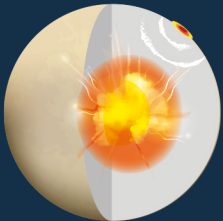
double detonation SN Ia
