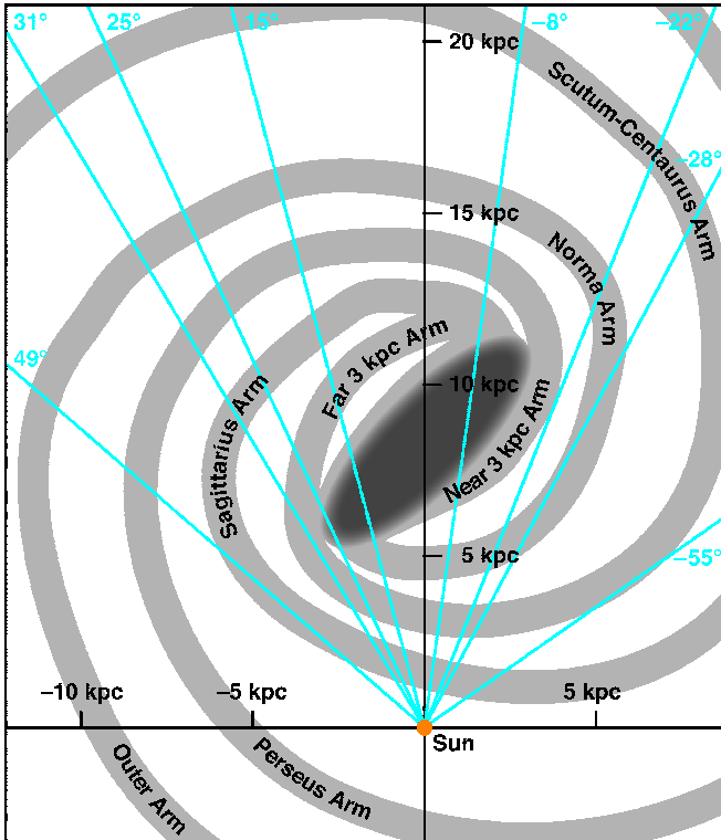
FIG. 3.— Sketch of the Galactic plane with several prominent lines of sight marked. Artist impression (by MPIA graphics department) of face-on view of the Milky Way following the Galactic structure discussed in Reid et al. (2009).
