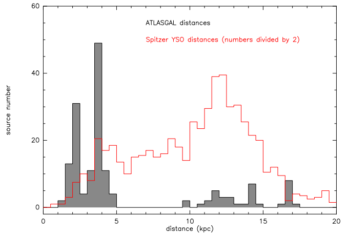
FIG. 1.— Histogram of distances derived for the ATLASGAL clumps (black, only the starless clumps) and the GLIMPSE YSOs (red) in the Galactic longitude range from 10 to 20 deg, respectively (Tackenberg et al. subm. , Robitaille & Whitney 2010).
