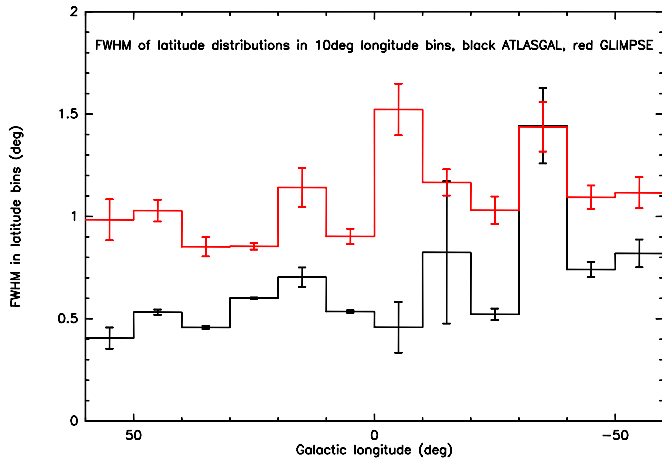
FIG. 6.— Resulting FWHM of Gaussian fits (and associated errors) to the latitude distribution in 10deg Galactic longitude bins. The black histogram is from the ATLASGAL data, and the red histogram from the GLIMPSE data.
