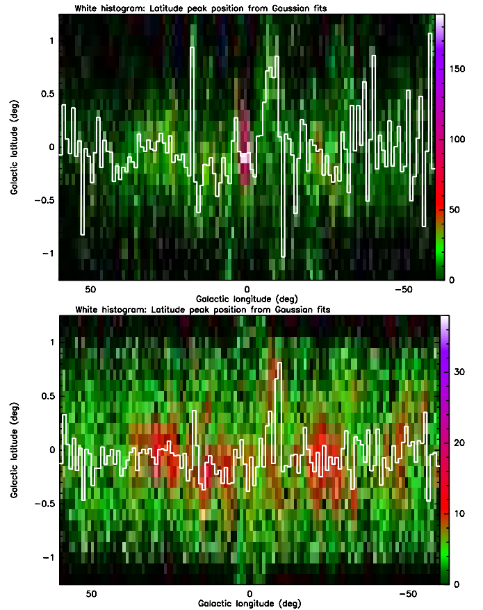
FIG. 4.— The color-scale shows the two-dimensional source count distribution for ATLASGAL submm continuum (top panel) and GLIMPSE YSO (bottom panel) sources. The bin sizes in Galactic longitude and latitude are 1 and 0.1 deg, respectively. The white lines mark the peak positions of Gaussian fits to the latitude distributions at each given longitude.
