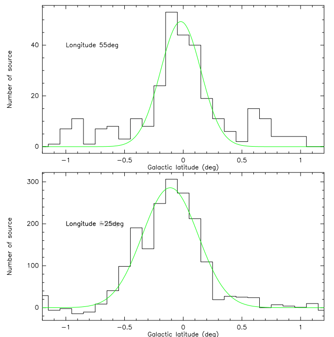
FIG. 5.— Examples of the Gaussian fits to the latitude distributions. The centers of the 10 deg longitude bins are labeled in each panel.
