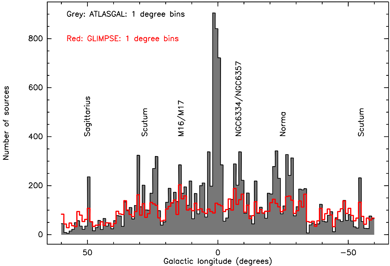
FIG. 2.— Histogram of source number counts with Galactic longitude. The grey-scale shows the ATLASGAL submm continuum sources, and the red histogram presents the YSOs derived from the Spitzer data (Robitaille et al. 2008). The data are binned in longitude in 1 deg bins. For ATLASGAL we use the data for latitudes between \pm 1.25 deg whereas the GLIMPSE YSO data are restricted to latitudes between \pm 1.0 deg.
