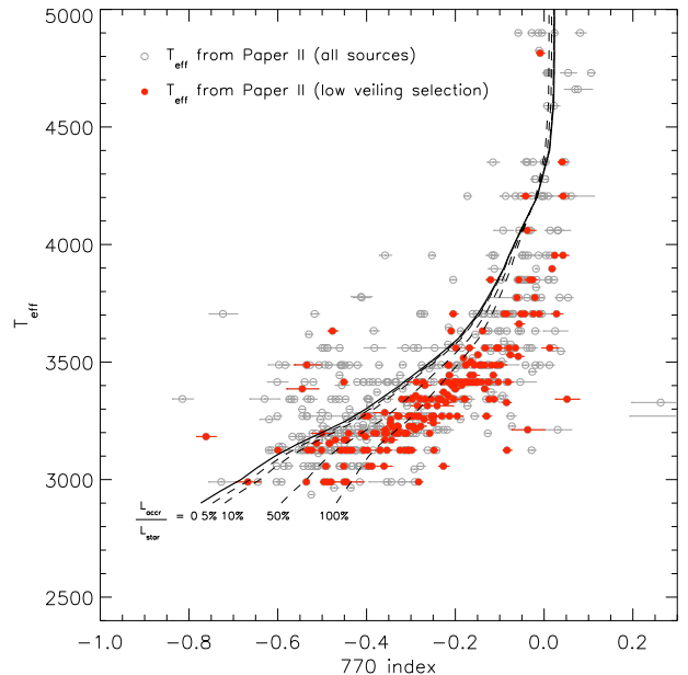
FIG. 9.— Same as Figure 8, showing the displacement in the reddening-independent [770 \text{ index}] obtained by adding an amount of accretion luminosity to the star. The thick line is the isochrone from Paper II, the same model shown also in Figure 5. The dashed line are the same model, after the addition of a given amount of accretion luminosity to the each synthetic spectrum, for different values of \log L_{\text{accr}}/L_{\text{tot}} . Note that the fact that the red dots are low accretion sources, whereas the model requires a large value of L_{\text{accr}} to predict their colors, implies that the base isochrone needs adjustments (see text).
