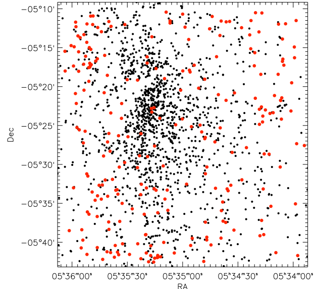
FIG. 15.— Spatial distribution of the ONC members placed in the H-R diagram (black dots). The red circles mark the position of the faint sources identified as background sources.
