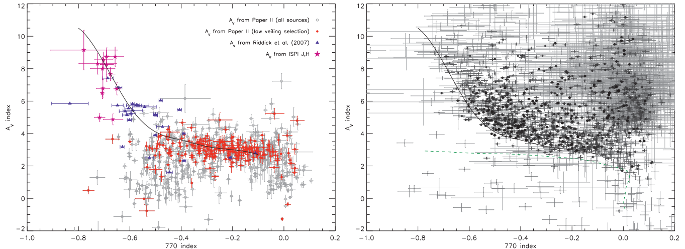
FIG. 11.— The color-color plot expressed in units of [770 \text{ index}] (reddening independent) and [A_V \text{ index}] (parallel to the reddening direction). Left panel: sample of extinction-corrected sources; A_V values are from Riddick et al. (2007), the JHK photometry of Robberto et al. (2010), and the optical analysis of Paper II. For the latter, accretors and candidate non accretors are distinguished as in Figure 8. The solid line represents our best fit of the data, i.e. the empirical isochrone for A_V = 0 . Right panel: same diagram, reporting all the sources in our catalog, with no correction for extinction. These are color coded according to their photometric errors. The entire population, with the exception of very few sparse sources, is located above the isochrone, at positive values of extinction.
