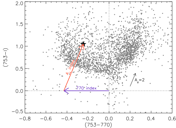
FIG. 7.— Conceptual scheme of the new coordinate system we introduce to measure T_{\text{eff}} and A_V of the stars from our color-color diagram: the T_{\text{eff}} dependent [770 \text{ index}] , and the reddening dependent A_V index. See text.
