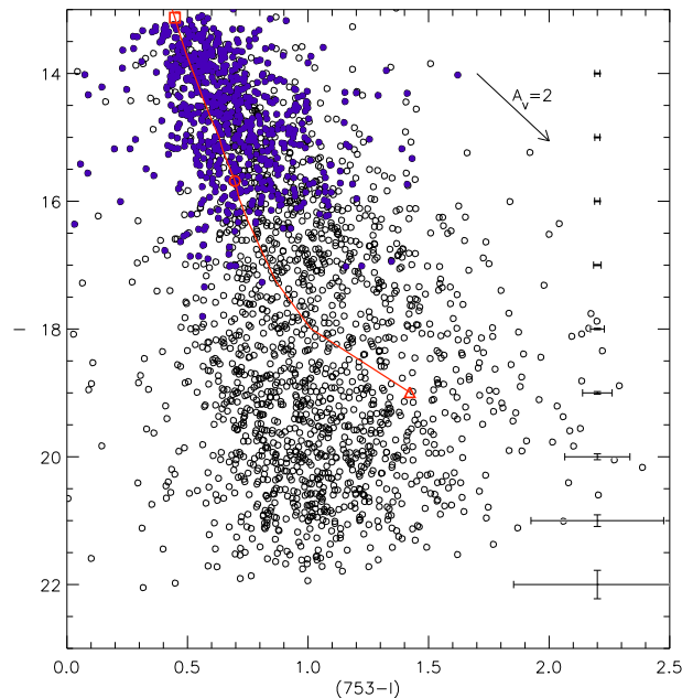
FIG. 4.— Open circles: the derived I vs 753 - I CMD including only the sources measured in all the 3 bands (i.e. also in 770). The filled blue circles indicate the sources included in our previous study of the stellar population of the ONC, based on WFI photometry and spectroscopy down to the H-burning limit (Paper II). The average photometric errors as a function of I -band are indicated to the right. The red line represents a 1 Myr Baraffe et al. (1998) isochrone; the square, circle and triangle symbols along the line mark masses of 0.4 M_{\odot} , 0.08 M_{\odot} and 0.02 M_{\odot} . The arrow denotes the reddening vector for A_V = 2 assuming the Cardelli et al. (1989) reddening law for R_V = 3.1 .
