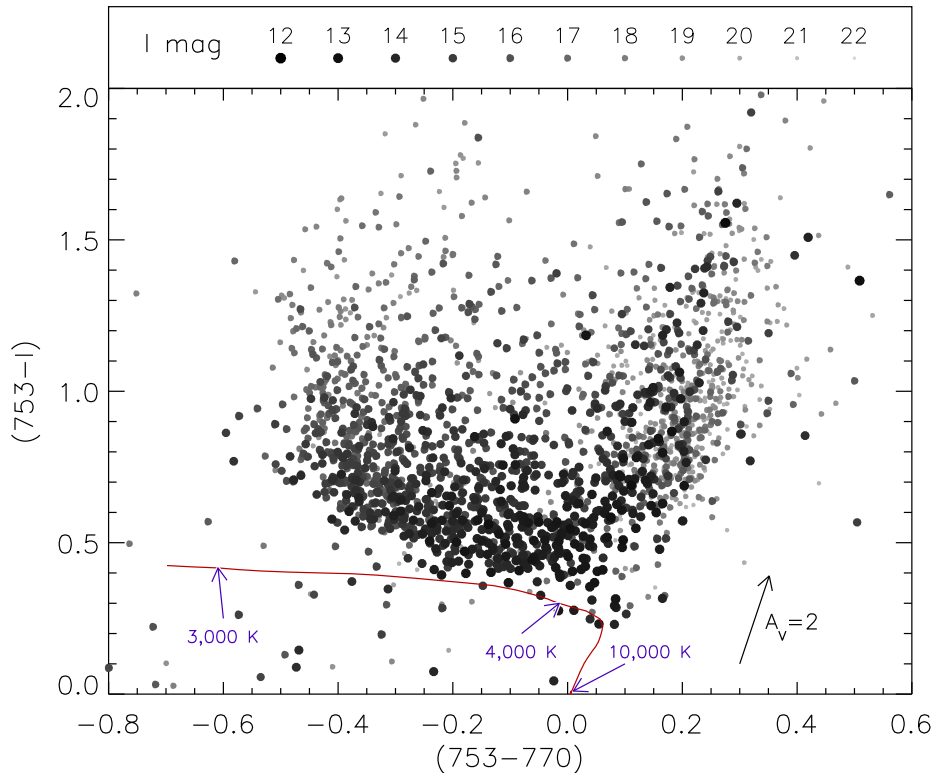
FIG. 5.— (753-I) vs. (753-770) color-color diagram from our photometry. The color and size of the dots indicates the I-band luminosity of each source, as indicated. The black arrow indicates the direction of the reddening vector for 2 mag of extinction in V -band, assuming the reddening law of Cardelli et al. (1989) for R_V = 3.1 . For reference, the thick red line is the empirical isochrone derived in Paper II converted in this color-color plane using the atmosphere models of Allard et al. (2000). For guidance, the origin (0,0) corresponds to 10,000 K, and the turn-over in (753-770) corresponds to T_{\text{eff}} \sim 4000 K, i.e. between K and M spectral classes.
