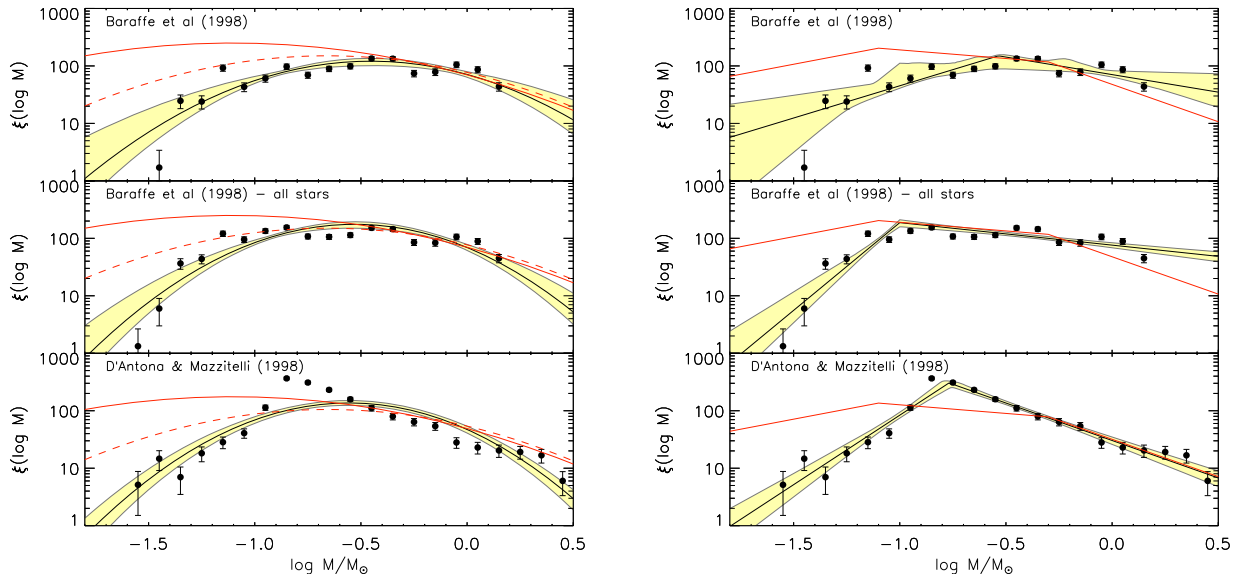
FIG. 18.— The measured IMF for the ONC, fitted with a log-normal distribution (left panel) or a two-phase power law (right panel). The top and bottom panels represent the mass distributions obtained assuming Baraffe et al. (1998) and D’Antona & Mazzitelli (1998) models respectively, whereas the center panels show the result assuming Baraffe et al. models and including also stars located above the 1 Myr, whose mass has been extrapolated from their T_{\text{eff}} (see text). The shaded areas enclose the 90% confidence interval for each fit. The red curves represent the IMF of Chabrier (2003) (left panel) and Kroupa (2001) (right panel); the red dashed line is the Chabrier (2003) system IMF.
