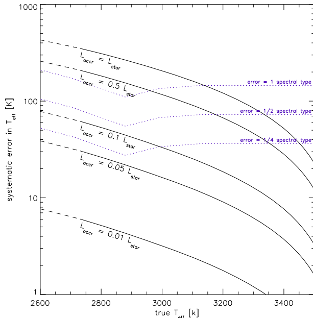
FIG. 10.— Computation of the offset on the derived T_{\text{eff}} , as a function of temperature, produced by neglecting accretion veiling. The solid lines represent the result for different accretion luminosities. The dotted lines represent the uncertainty in T_{\text{eff}} associated to an uncertainty in the spectral type of 1 subtype, half subtype and 1/4 of a subtype.
