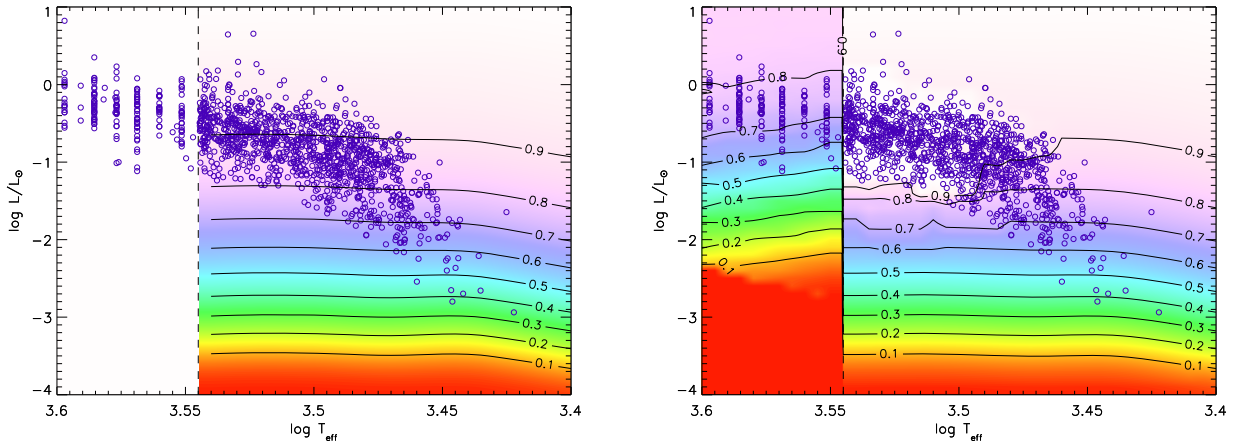
FIG. 17.— Completeness function in the H-R diagram, computed accounting for photometric detection and differential reddening as described in the text. The left panel shows the result as computed with our monte-carlo simulation, valid for the spectral types obtained from the medium-band photometry analyzed in this work, for \log T_{\text{eff}} < 3.54 ( T_{\text{eff}} < 3500 K). The right panel shows the correction of this completeness after accounting for the additional stars placed in the HRD whose stellar parameters are taken from Paper II.
