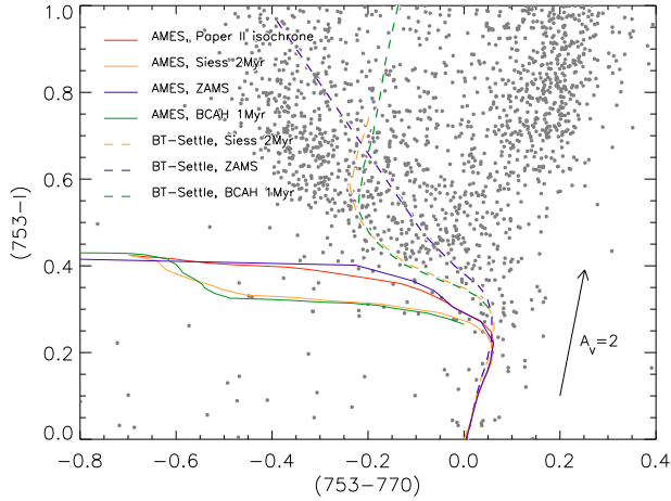
FIG. 6.— The color-color diagram of Figure 5, with different synthetic isochrones overplotted. In particular: a Siess et al. (2000) 2 Myr isochrone; a Baraffe et al. (1998) 1 Myr isochrone; a Siess et al. (2000) zero-age main sequence. Thick lines are the result from synthetic photometry on the AMES-MT grid of spectra from Allard et al. (2000), while dashed lines are computed using the BT-Settle grid from Allard et al. (2010). The thick red line is computed using the empirical calibration of the AMES-MT models defined in our Paper II to match the broad band BVI colors of the ONC. The empirical line is actually closer to the predicted ZAMS relation than the predicted 1-2 Myr isochrones, illustrating the current lack of agreement between evolutionary and atmosphere models and young star photometry (see text).
