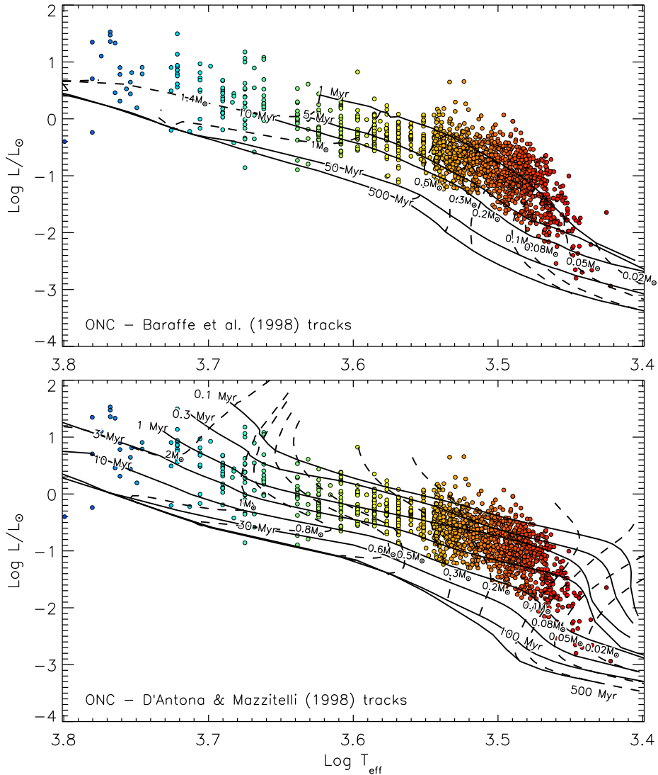
FIG. 16.— The H-R diagram of the ONC members, after the removal of contamination from background stars. Evolutionary models are from Baraffe et al. (1998) (upper panel) and D’Antona & Mazzitelli (1998) (lower panel).
