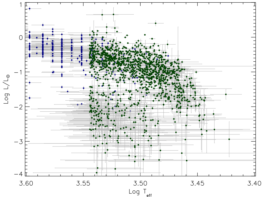
FIG. 13.— The new H-R diagram of the ONC. Green dots are the new stars whose stellar parameters have been derived in this work, blue dots are members from Paper II, mostly having a large enough T_{\text{eff}} to not be derivable using the [770 index ], or saturated in our new WFI photometry.
