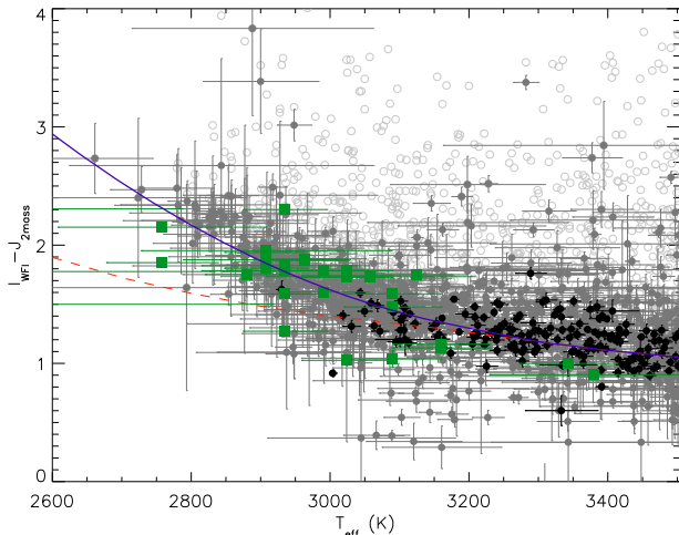
FIG. 12.— (I - J) vs T_{\text{eff}} : the open dots are the measured colors, the filled gray dots are the de-reddened ones. Black dots are de-reddened colors for sources with known estimate of accretion excess, showing no significant excess. Green squares are sources whose T_{\text{eff}} is from Riddick et al. (2007). The dashed line is the prediction from synthetic photometry on the BT-Settle atmosphere models of Allard et al. (2010); the solid line is the empirical fit to the data.
