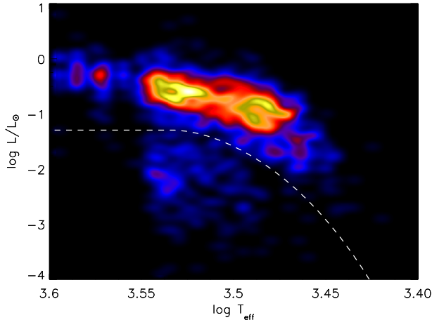
FIG. 14.— Stellar density map in the H-R diagram. The dashed line marks our adopted separation between bona fide members and contaminants.
