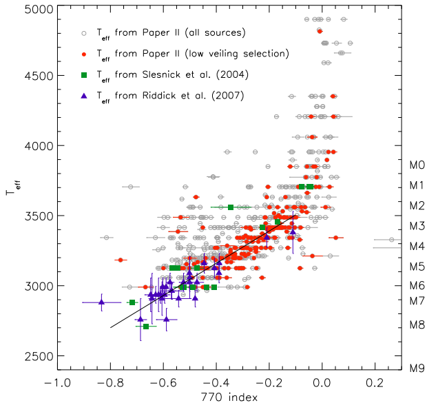
FIG. 8.— Derived relation between the measured, reddening independent, photometric [770 \text{ index}] , and spectroscopically determined stellar temperature. The values of T_{\text{eff}} for the stellar mass regime ( T_{\text{eff}} \gtrsim 3000 \text{ K} ) are from the spectral types collected in our Paper II. For these sources, we identify a sample of candidate weak accretors, showing low H\alpha emission ( E.W. < 10\text{\AA} ) and no significant veiling ( \log L_{\text{accr}}/L_{\text{tot}} < -1.5 ), in order to more cleanly determine the true relationship between the photometric [770 \text{ index}] and T_{\text{eff}} . Spectroscopic T_{\text{eff}} for substellar masses are from Riddick et al. (2007) and Slesnick et al. (2004). See text for details.
