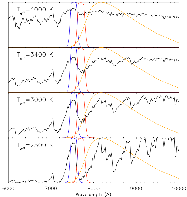
FIG. 1.— The band profiles of the 3 WFI filters used in this work (from left to right: 753, 770 and I –band) overlaid to spectra of very low-mass stars (4000 K to 3000 K) and BDs (3000 K to 2500 K) from Allard et al. (2000).
